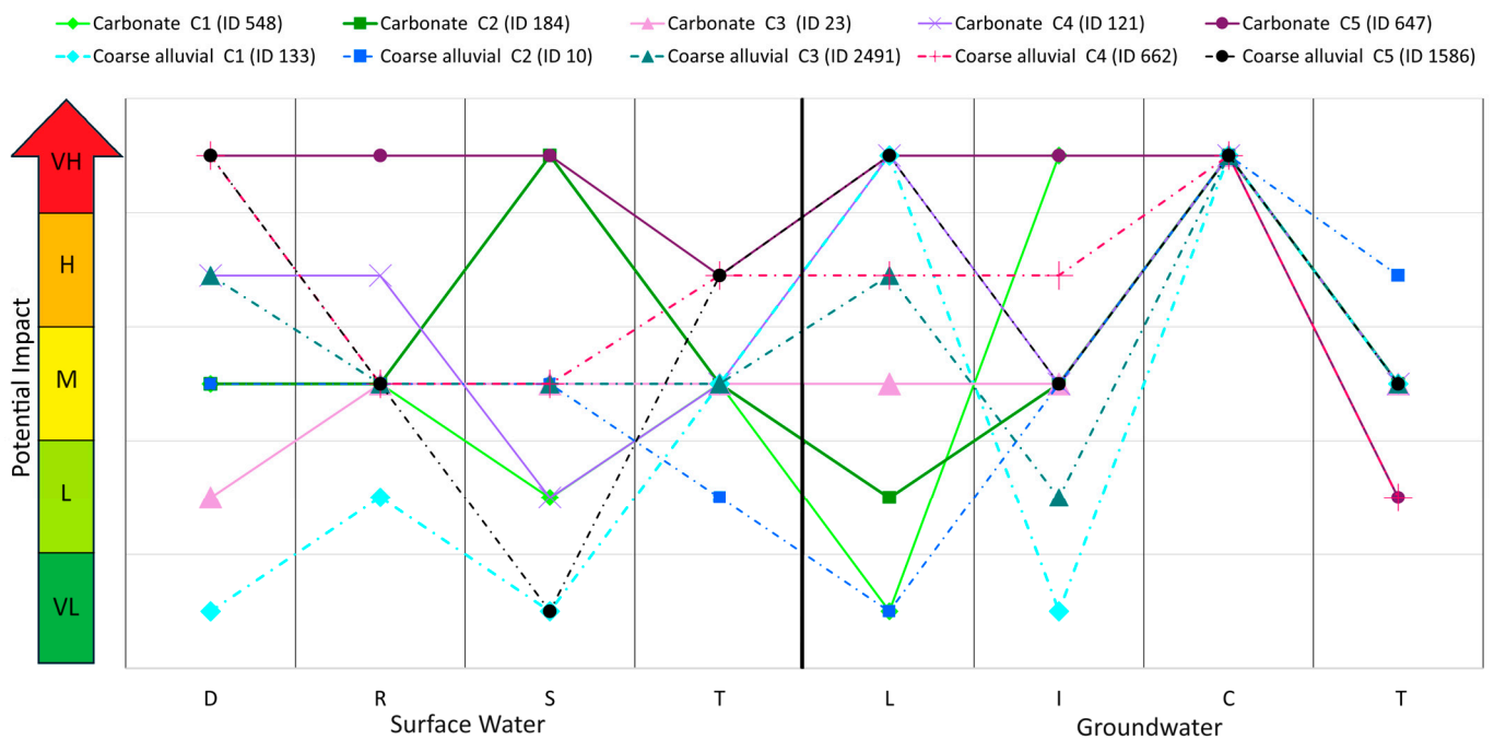
Figure 7. Examples of quarry categorization and its dependence on the different selected criteria.
