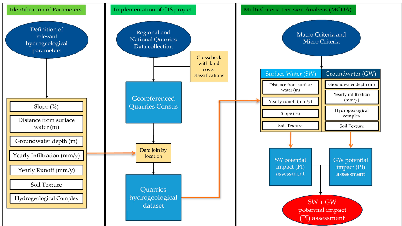
Figure 1. Flowchart of categorization of Italian quarries depending on their potential impact on water resources.
