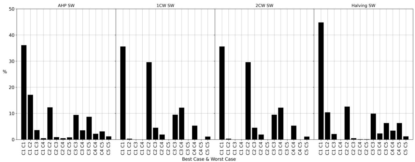
Figure 8. Percentage distribution of quarries in different categories for the potential impact on surface water resulting from the four simulations (AHP, 1CW, 2CW, and halving models of micro-criterion weights).
