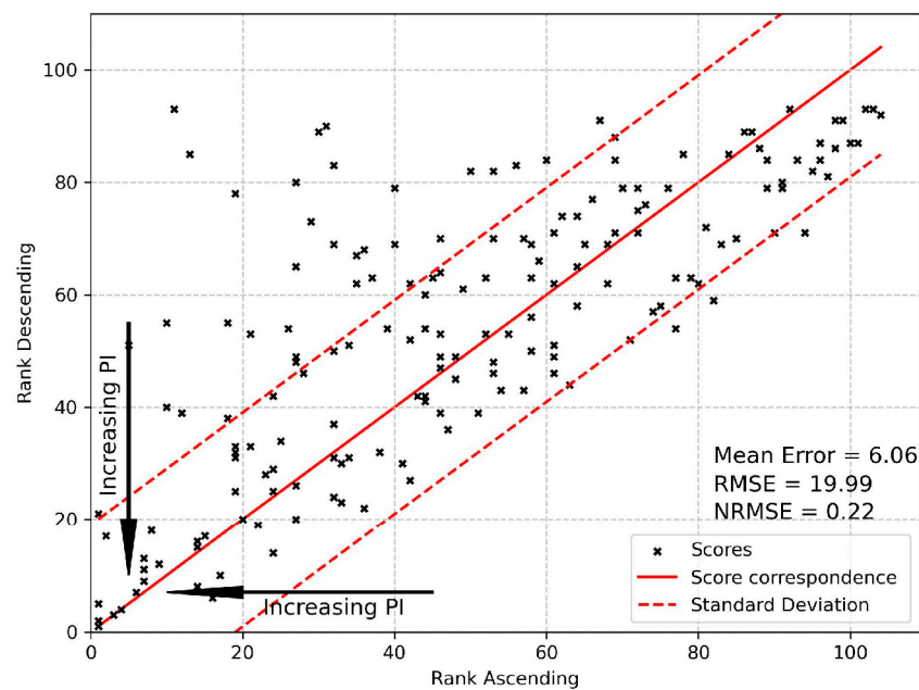
Figure 11. Comparison of ranking of potential impact on water resources (PI) of ascending and descending distillations for the two categories C4-C5 and C5 (halving model for the micro-criteria weights).
