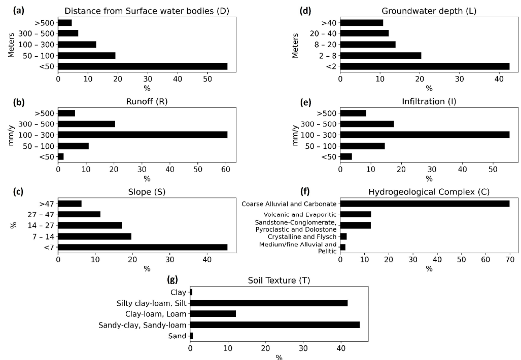
Figure 6. Percentage distribution of the classes related to the seven parameters considered for the MCDA model: (a) distance from surface water (D); (b) runoff (R); (c) slope (S); (d) depth of groundwater level (L); (e) effective infiltration (I); (f) hydrogeological complex (C); (g) soil texture (T).
