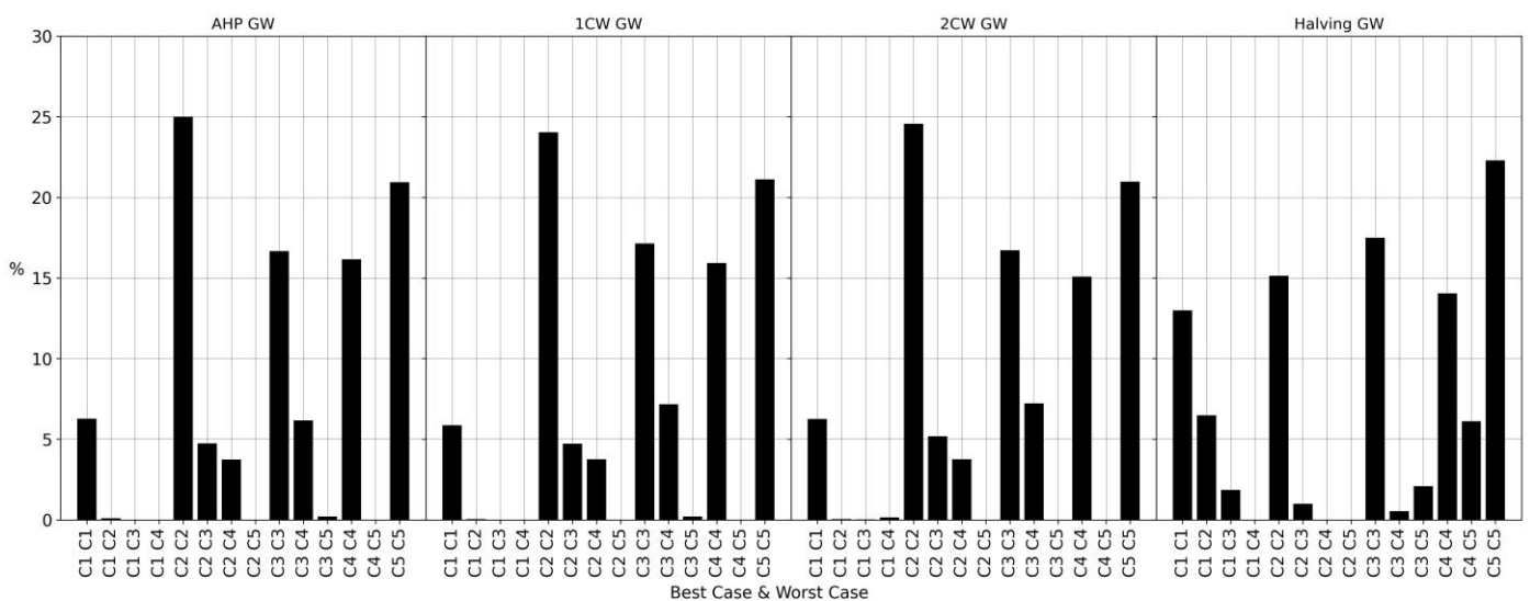
Figure 9. Percentage distribution of quarries in different categories for the potential impact on groundwater resulting from the four simulations (AHP, 1CW, 2CW, and halving models of micro-criterion weights).
