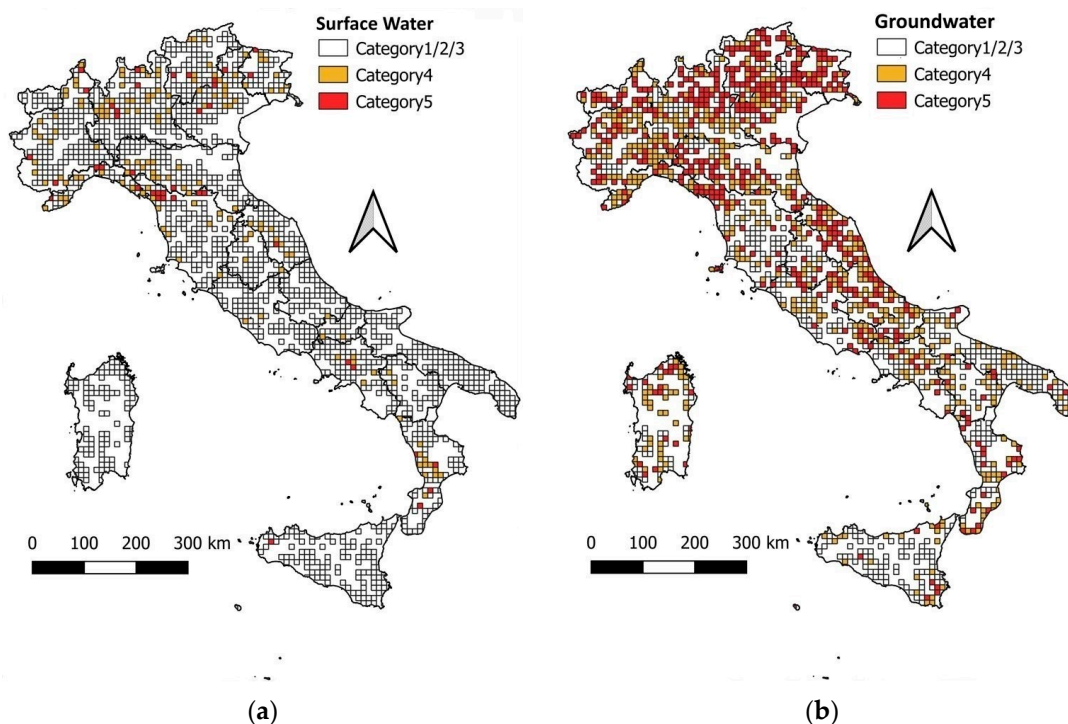
Figure 12. Distribution of quarries into different categories of potential impact on (a) surface water and (b) groundwater (halving model of weights).
