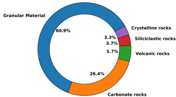
Figure 5. Percentage distribution of materials extracted in Italy.
