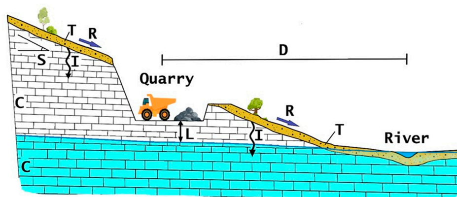
Figure 2. Conceptual scheme of parameters influencing the impact of quarries on water resources: D, distance from surface water body; R, runoff; I, effective infiltration; S, slope; C, hydrogeological complex; L, depth of groundwater level; T, soil texture.
