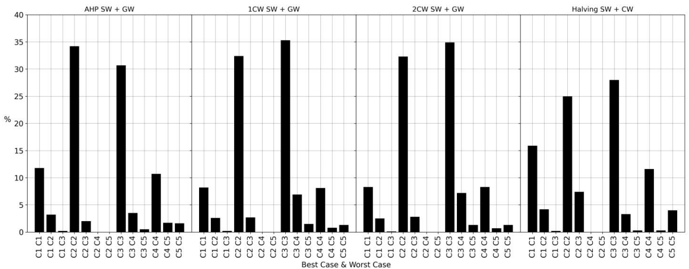
Figure 10. Percentage distribution of quarries in different categories for the potential impact on water resources resulting from the four simulations (AHP, 1CW, 2CW, and halving models of micro-criterion weights).
