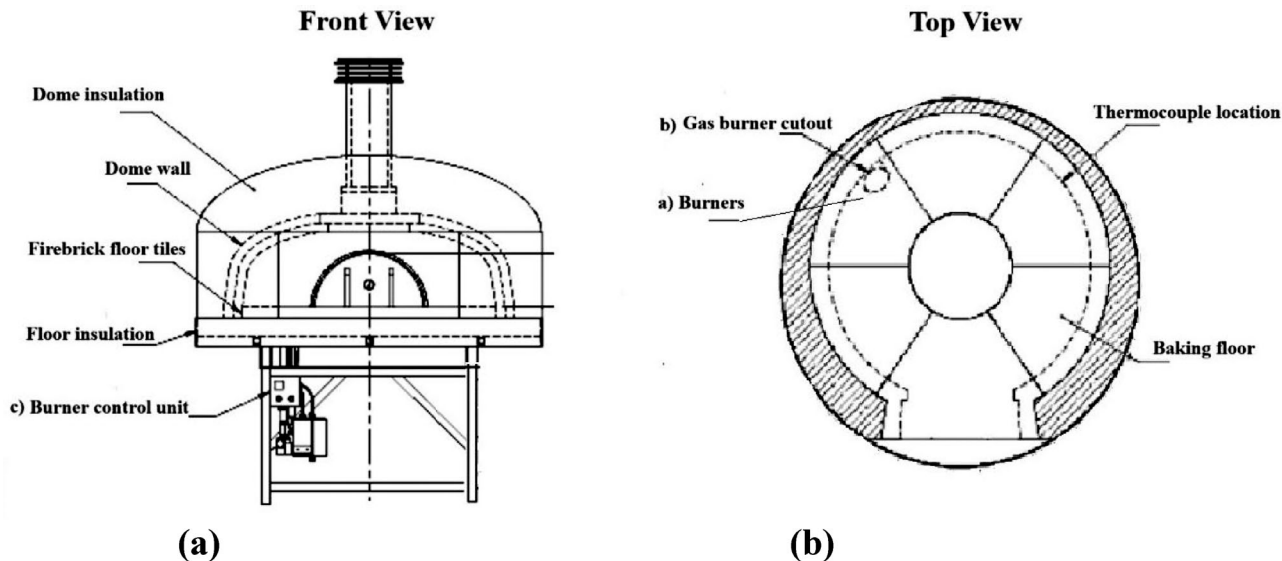
FIGURE 9 Front view (a) and top view (b) of a typical gas pizza oven, freely reinterpreted from the online catalogs of the pizza oven manufacturers mentioned in the text, with its main components labeled: a) burners, b) gas burner cutout, and c) burner unit control.
