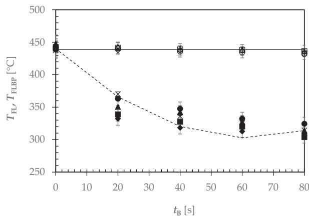
FIGURE 5 Effect of baking time ( t_B ) on the average temperatures of the oven floor exposed to the fire ( T_{FL} : empty symbols; +) or shielded by the pizza ( T_{FLbp} : closed symbols, X) as determined by Falciano et al. (2023b) during the baking tests of various types of pizza: white: \circ , \bullet ; white with oil: \triangle , \blacktriangle ; tomato: \square , \blacksquare ; tomato with oil: \diamond , \blacklozenge ; tomato with oil and mozzarella: +, X. The solid horizontal line indicates the average temperature of the oven floor around any pizza during baking, whereas the broken line represents the temperature profile of the oven floor covered by a tomato pizza.
