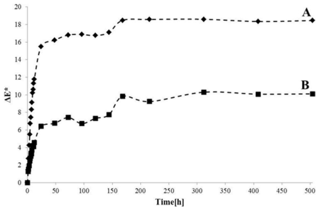
Figure 2. Changes in \Delta E^* values due to exposure in Solar Box of the normal (A) and red heart wood (B) over 504h.
