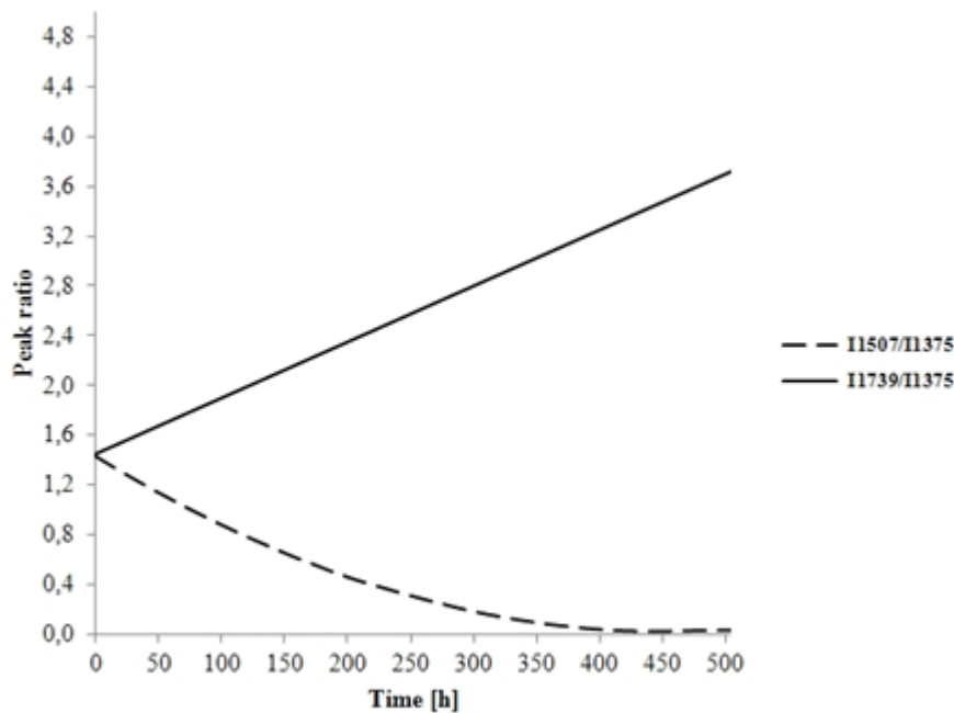
Figure 6. Change in the ratio band at different exposure times, as calculated from the regression analysis shown in Table 6.
