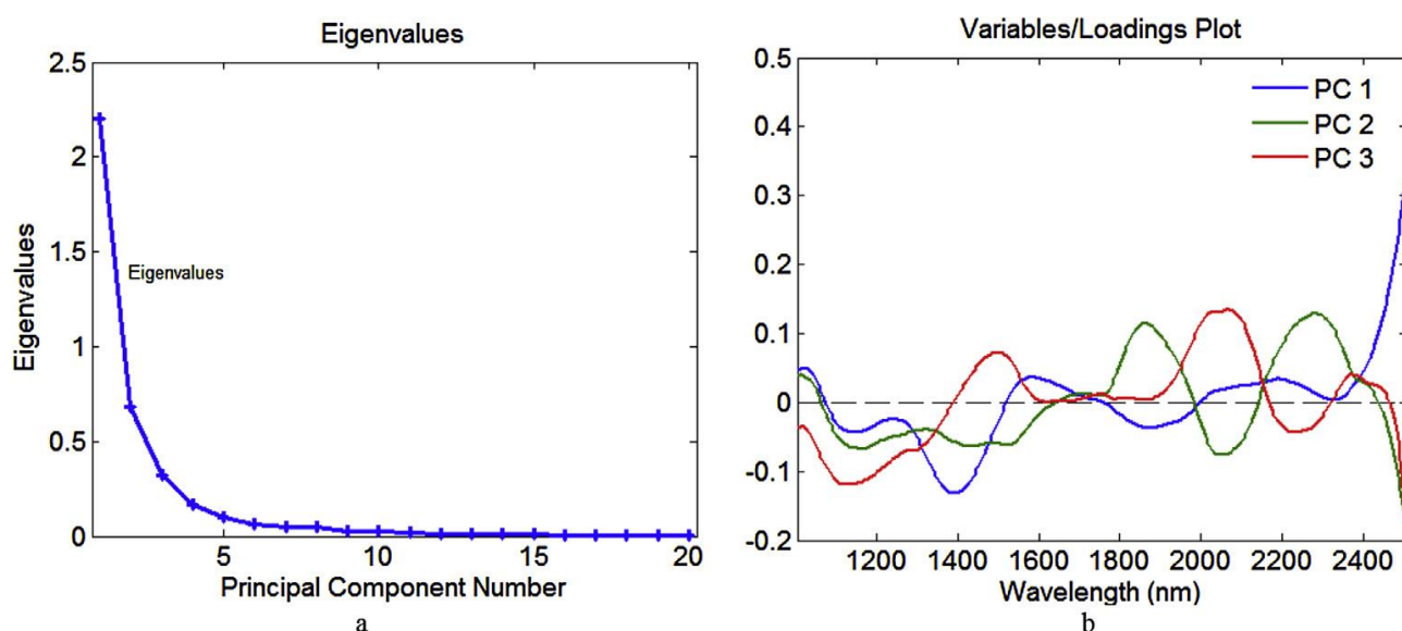
Figure 12. a: Eigenvalues for all PCs. b: Loadings of the selected PCs.
