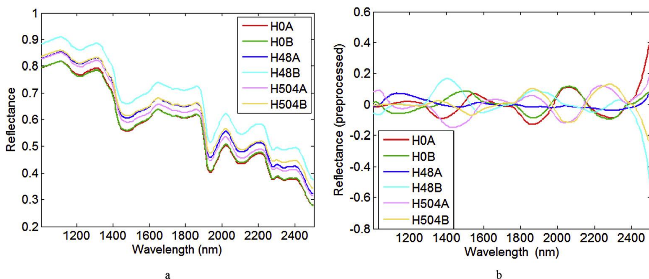
Figure 11. a: Average reflectance spectra of red heart (A) and normal (B) wood characterized by 3 different exposure times (H0, H48 and H504) acquired in the SWIR range. b: Corresponding preprocessed spectra after the application of 1st Derivative, SNV and mean center. (For interpretation of the references to colour in this figure legend, the reader is referred to the web version of this article.)
