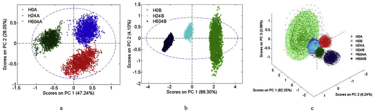
Figure 10. a: PCA score plot (PC1 vs. PC2) of red heartwood (A); b: PCA score plot (PC1 vs. PC2) of normal wood (B); c: PCA 3D score plot (PC1, PC2 and PC3) of both wood sample typologies in the VIS-NIR range.
