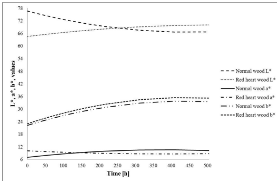
Figure 3. Colour changes of normal and read heart wood due to irradiation. L*, a* and parameters at different exposure times as calculated from the regression analysis shown in Table 2.
