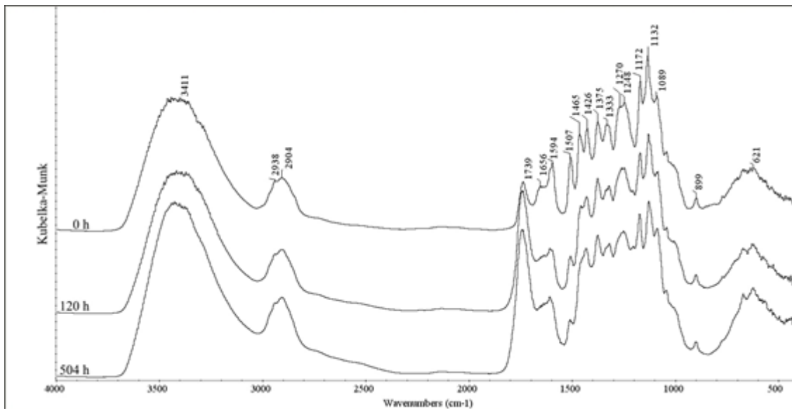
Figure 4. Diffuse reflectance spectra of normal wood slices measured at chosen exposure times
