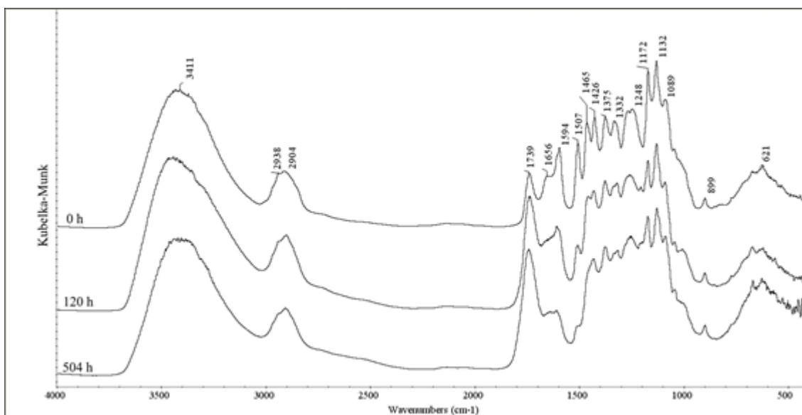
Figure 5. Diffuse reflectance spectra of red heartwood slices measured at chosen exposure times.
