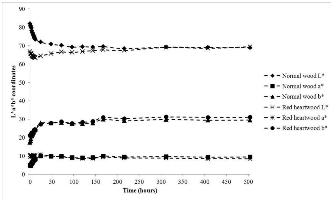
Figure 1. Changes in L*a*b* values due to exposure in Solar Box of the normal and red heart wood over 504h.
