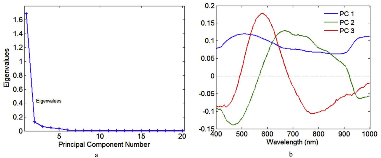
Figure 9. a: Eigenvalues for all PCs. b: Loadings of the selected PCs.
