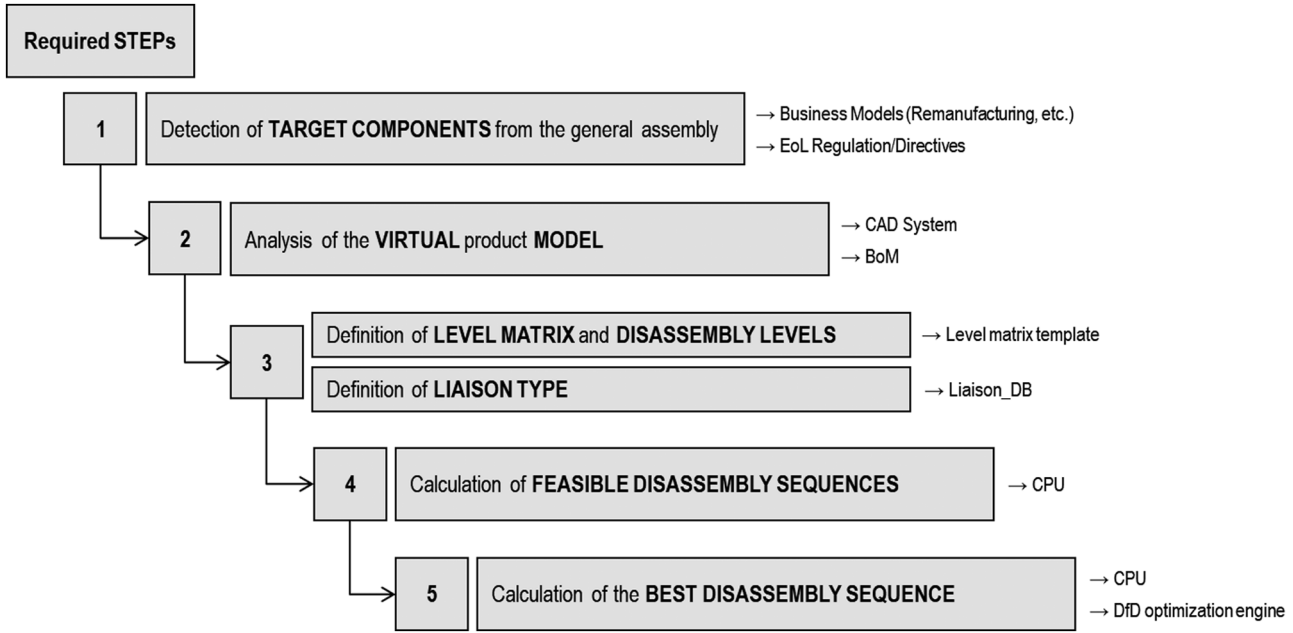
Figure 1. Workflow of the proposed DSP approach.
