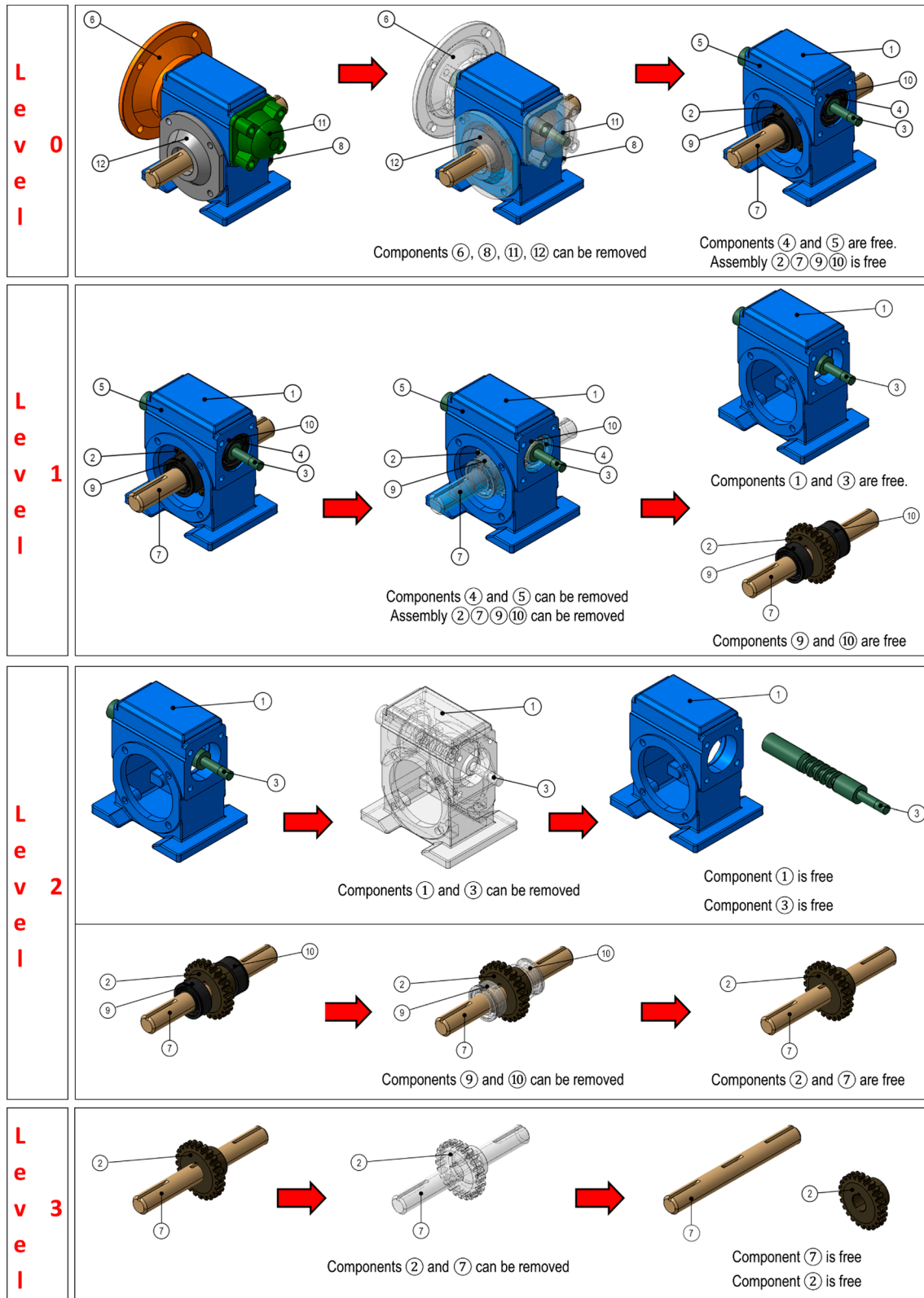
Figure 3. Disassembly levels for the gear reducer example.
