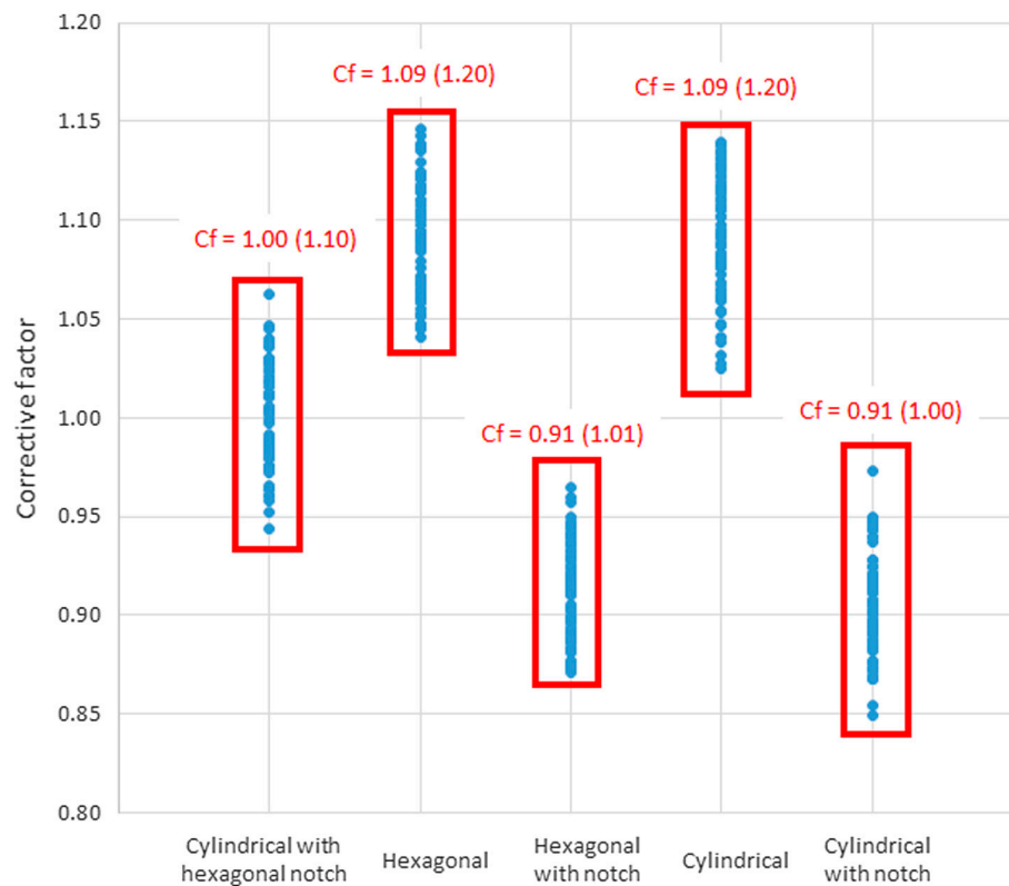
Figure 8. Corrective factors for screw head type (cluster view). Within brackets the normalised corrective factors.
