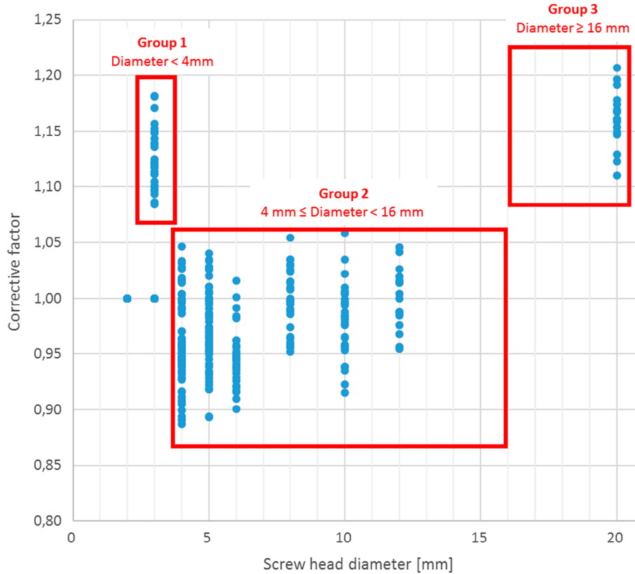
Figure 6. Screw diameter clustering (k-means algorithm).
