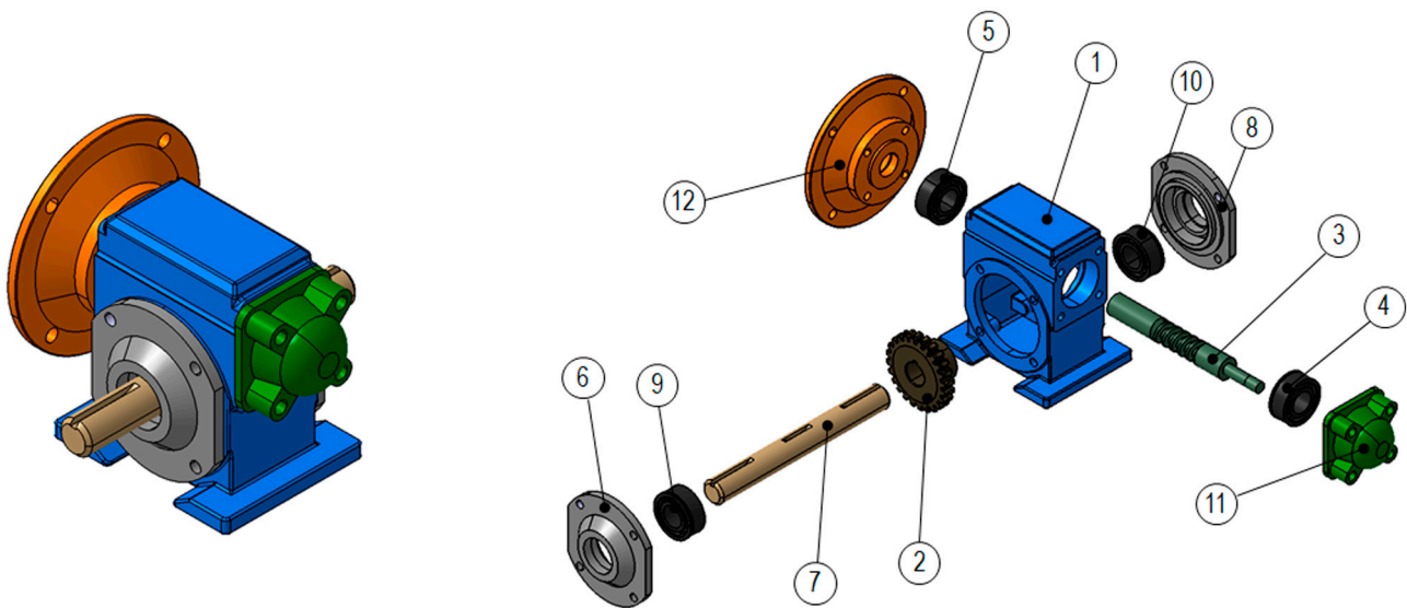
Figure 2. Exploded view of the gear reducer example.
