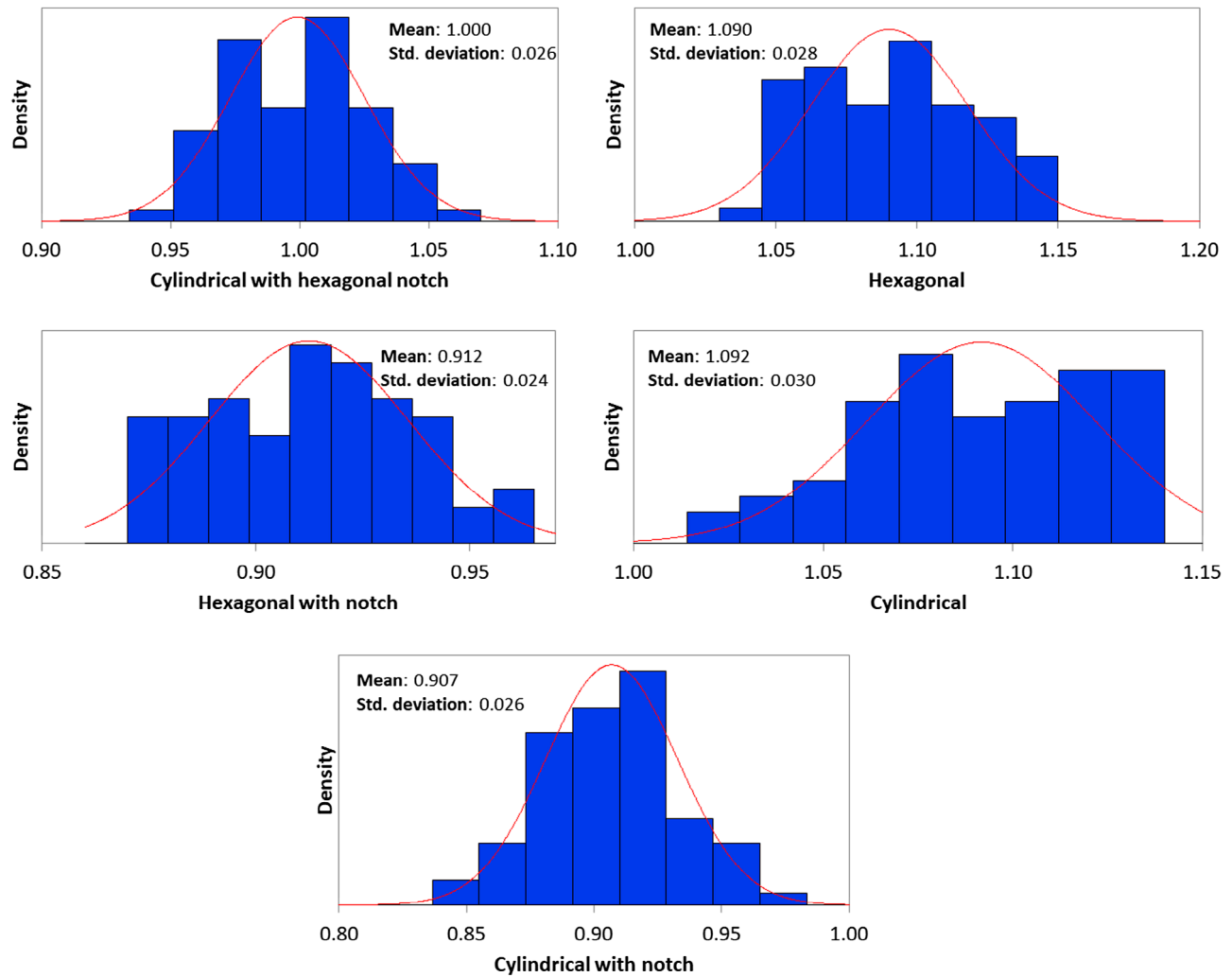
Figure 9. Distribution fitting analysis for the corrective factors.
