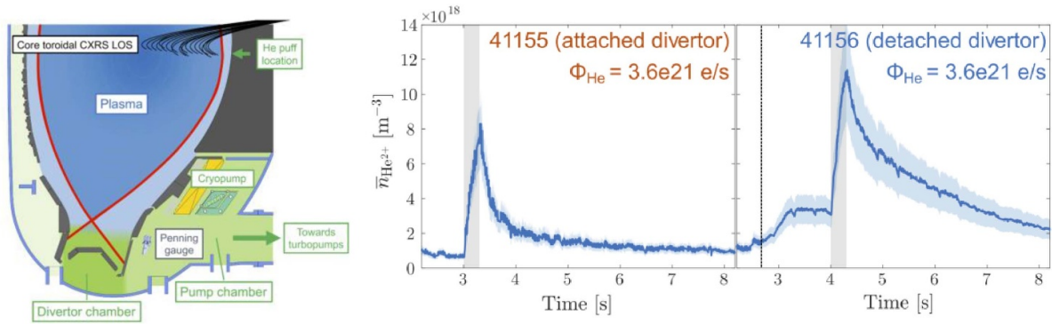
Figure 7. Study of He pumping in AUG: simultaneous measurement of the core He density by CXRS and the neutral density in the pump chamber using a Penning gauge allows to study the enrichment of He. The left panel shows the experimental setup, the right panels show the decay of the core He density after a He gas puff in attached and detached divertor conditions, indicating that the He pumping is less efficient in detached conditions.
