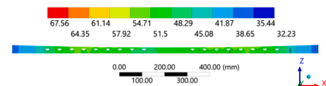
Fig. 15. Copper mirror: contour plot of the temperature distribution on the section view with the scale of the previous case.
