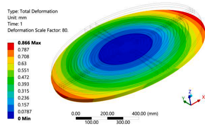
Fig. 13. Contour plot of the total deformation of the SS-Cu (spiral) mirror design. Deformation scale factor (x80).
