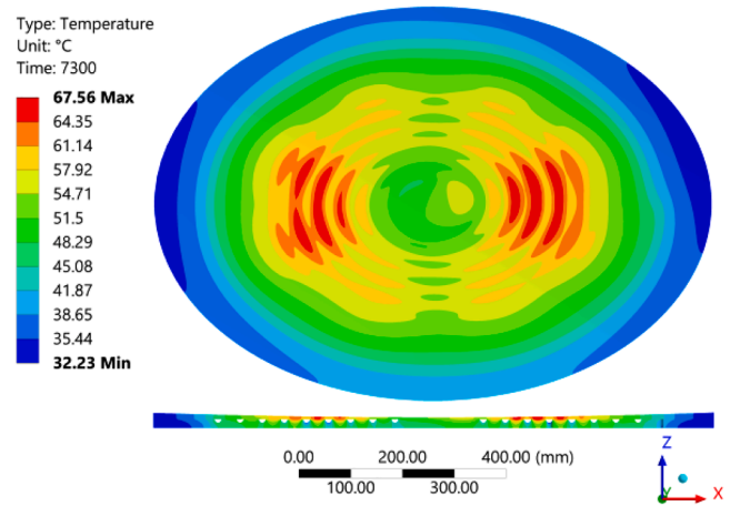
Fig. 11. SS-Cu (Spiral) mirror: (Top) Contour plot of the temperature distribution at the end of the third pulse, front view. (Bottom) Temperature distribution on the section view (x-z plane).
