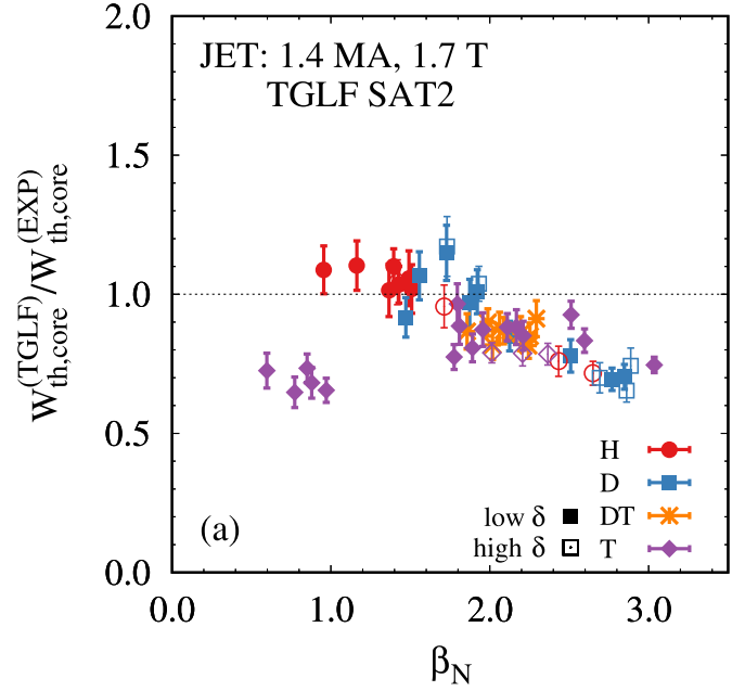
Figure 20. Comparison of ASTRA-TGLF (SAT2) predictions of core thermal stored energy W_{th,core} and experimental value W_{th,core} (EXP) = W_{th} - W_{th,ped} vs \beta_N showing increasing underprediction by ASTRA-TGLF with increasing \beta_N . Tritium data at \beta_N \sim 1 are shown for comparison (although not in type I ELMy regime). Reproduced from [96]. © 2023 The Author(s). Published by IOP Publishing Ltd on behalf of the IAEA. All rights reserved. CC BY 4.0.
