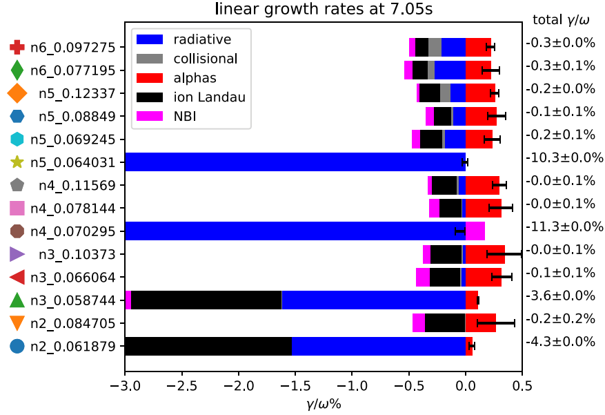
Figure 12. Contributions by drive and damping to linear growth rates \gamma/\omega of various TAE modes calculated by MISHKA from JET D–T pulse #99946, indicating \alpha -driven TAE observation for a mode with n = 3 or n = 4 . Reproduced from [76]. © 2023 Crown copyright, UKAEA. CC BY 4.0.
