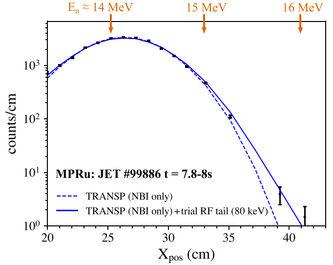
Figure 26. Neutron spectrum measured with the upgraded magnetic proton recoil spectrometer (black points) and comparison with spectra from TRANSP simulations with only NBI slowing down (dashed blue line) and with NBI + trial RF tritons tail (solid blue line), with tail temperature of 80 keV (JET D–T hybrid discharge #99886). Reproduced from [117]. © 2023 The Author(s). Published by IOP Publishing Ltd on behalf of the IAEA. All rights reserved. CC BY 4.0 .
