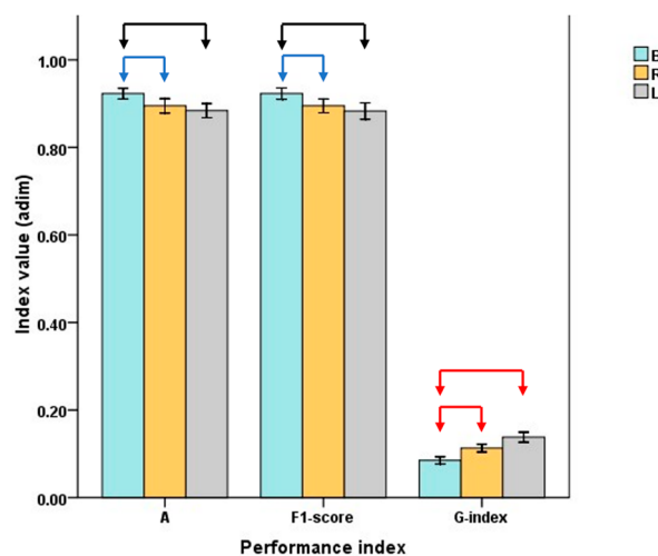
Figure 3. Mean and standard error of the performance index for the quadratic SVM. Arrows indicate the presence of a statistical difference between the type of dataset subsampling. Black, blue and red indicate p -values < 0.01 , = 0.05 and < 0.001 , respectively. B, R and L stand for Both, Right and Left, respectively.
