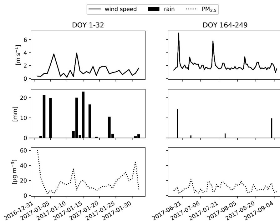
Figure 1. Wind speed, precipitation, and \text{PM}_{2.5} concentration throughout the two measurement campaigns. Particulate matter data are reported for the period DOY 1–32 up to the leaf sampling day (February 1st).
