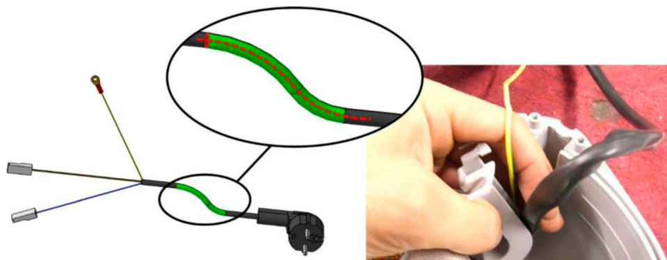
Figure 6. Identification of the critical product feature ( circular section sweep on polylines ) for the cable.
