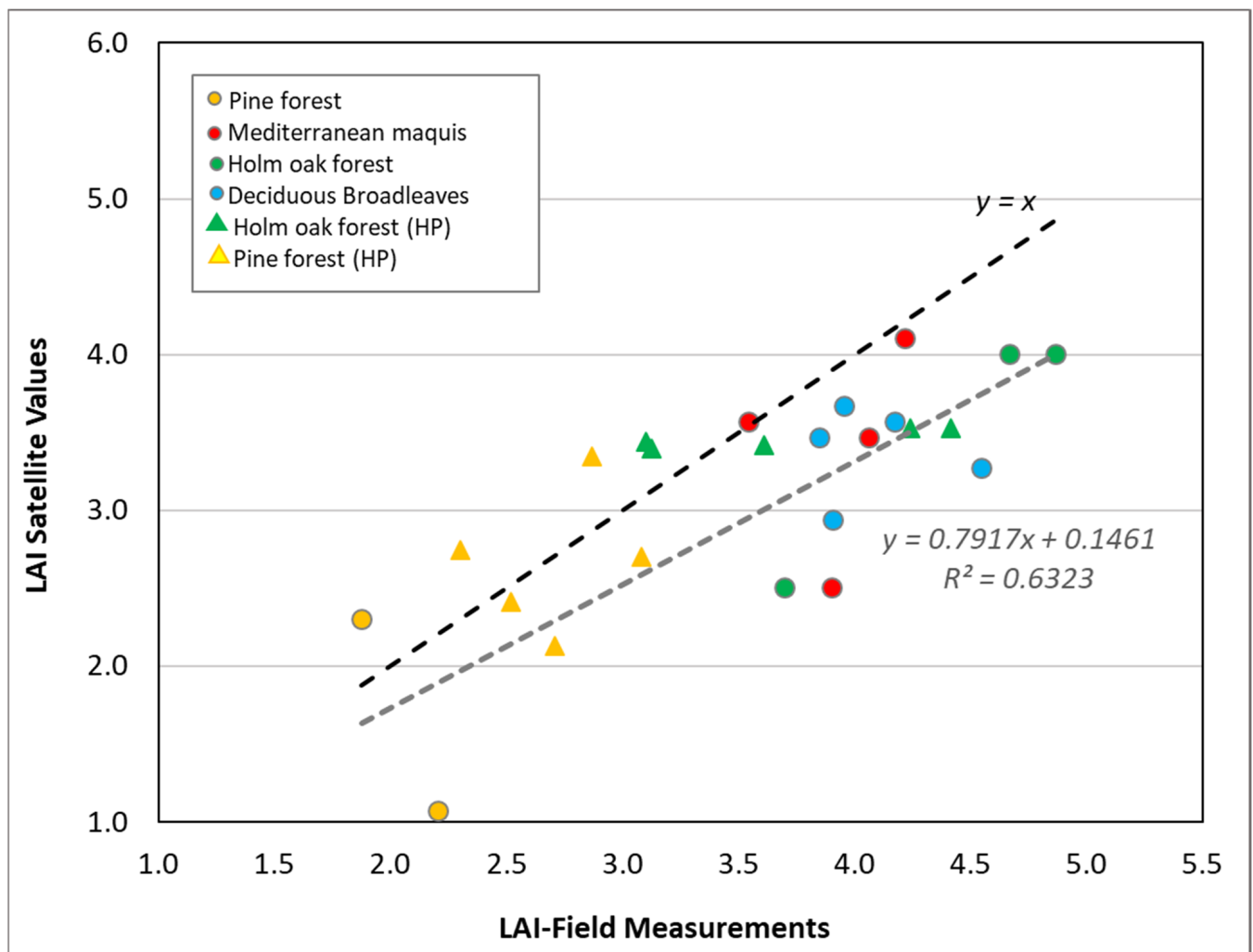
Figure 4. Correlation between ground-level measurement and satellite-level values of LAI ( \text{m}^2 \text{m}^{-2} ); different colors represent different LCT sampled inside the Estate. The circles indicate field measurements carried out with LAI-2200C Plant Canopy Analyzer; triangles indicate field measurements carried out with hemispherical photography (HP).
