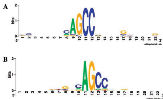
Fig. 2. Logo representation of the sequence alignment of regions spanning positions -10 to +10 surrounding the CC donor and the AG acceptor for 26 splice sites of 25 genes, supported by \geq 4 ESTs. The genome-EST alignments supporting such CC/AG splice sites are shown in Supplementary Fig. 3).
