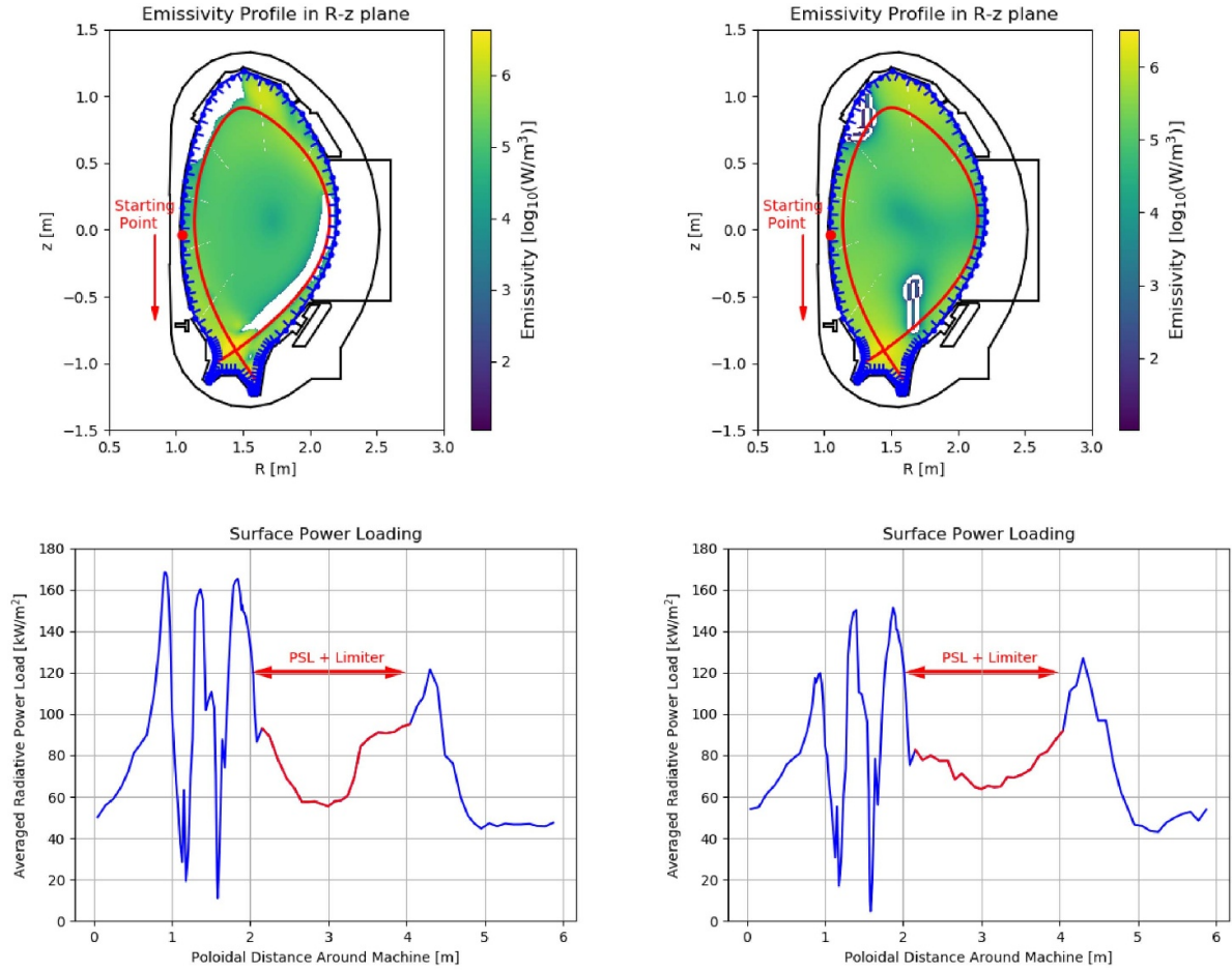
Figure 6. Overview of the setup used in CHERAB in order to assess the poloidal distribution of radiative energy loads for discharge #39231: left column with experimental 2D emissivity profile and obtained poloidal radiative heat load distribution, right column with simplified synthetic 2D emissivity profile and obtained poloidal radiative heat load distribution. The white artifacts in both emissivity profiles represents negative values, which are set to 0 in this study. The starting point and direction of the evaluation scheme is indicated in each top plot. The area of interest ‘PSL + Limiter’ is indicated in both poloidal distributions.
