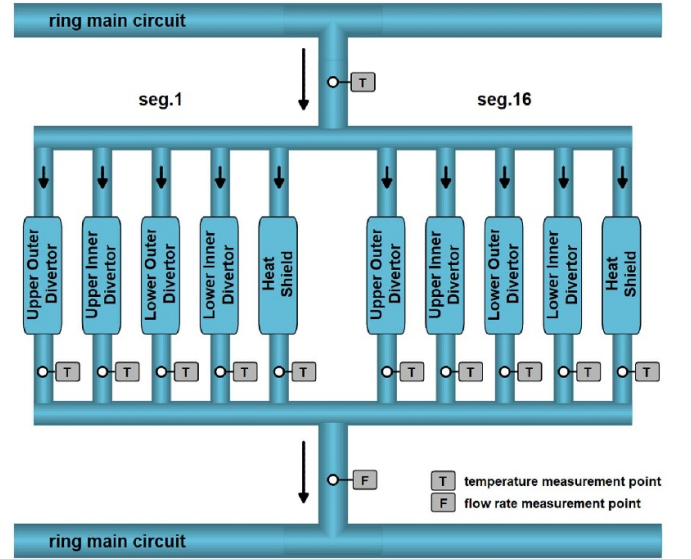
Figure 2. Simplified illustration of the cooling circuit of two segments (here segment 1 and 16). From the ring main circuit, the inlet cooling water temperature is measured before the cooling water is distributed to the individual cooling units of each segment. After leaving the vessel, the temperature of the outlet cooling water of the respective cooling units is measured. After merging the individual cooling tubes, the flow rate of the segment is measured.
