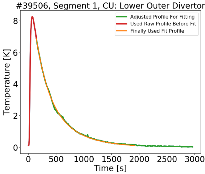
Figure 3. Plot of the \Delta T -profile for the cooling unit in the lower outer divertor in segment 1 for AUG discharge #39506. The green and red profile yield the original \Delta T -profile. The orange curve represents the extrapolated fit function (according to equation (2)) providing the full decay profile required for the calculation of the deposited energy in this cooling unit.
