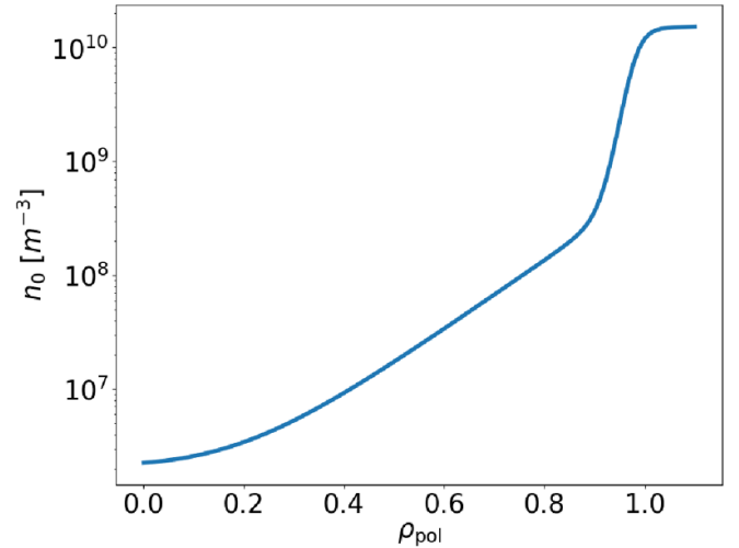
Figure 5. Visualization of the fit profile for the neutral particle density based on the fit introduced in [27]. The same fit profile is used for the entire database.
