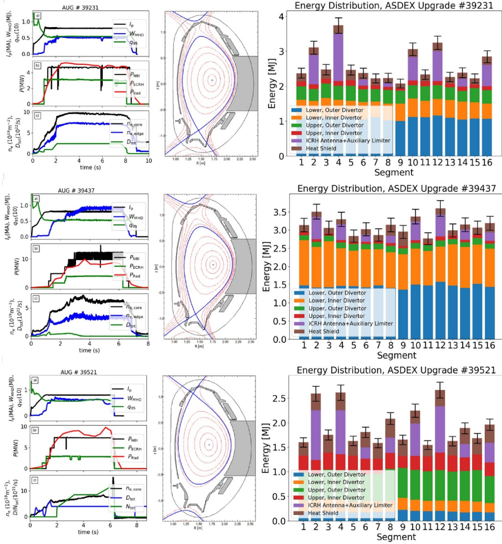
Figure 4. Overview of time traces of main plasma parameter, equilibrium at t = 4.0 s and the energy distribution calculated with the cooling water calorimetry for three different scenarios: top row represents the quantities of a QCE discharge (for more information concerning this discharge, we refer to [14], the middle one of an AT discharge [15] and the bottom one of an USN discharge in CRD configuration (for more information concerning this scenario, we refer to [16]). For this discharge, the edge density n_{e,edge} measured with the interferometer is not available. Instead, the nitrogen seeding rate N_{tot} is plotted. We want to emphasize that the scaling of the y-axis for each energy distribution is different.
