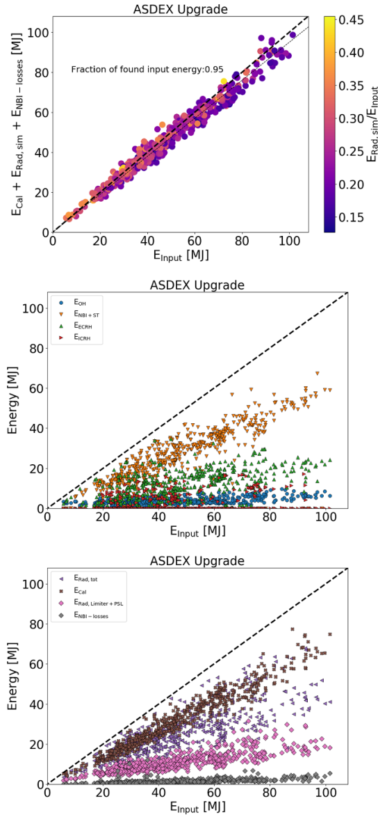
Figure 7. Top: Visualization of the global energy balance obtained with the optimized cooling water calorimetry at the AUG tokamak. The x-axis represents the left-hand side of equation (3), whereas the y-axis represents the right-hand side of that equation. A colormap is added representing the fraction of simulated radiative energy normalized against the injected energy for each discharge. Applying a linear regression on that database, one yields a detection rate of 95% of the input energy. Middle: Visualization of each contributor to the global energy balance of the left-hand side of equation (3). The four contributions represent the injected energy of each heating system available at AUG. Bottom: Visualization of each contributor to the global energy balance of the right-hand side of equation (3). The three contributions represent the calorimetrically captured energy, the simulated radiative energy reaching the limiter shadow and the PSL and contributions related to NBI losses. Additionally, the total radiative energy taken from the foil bolometry [30] is added as comparison for the simulated contribution.
