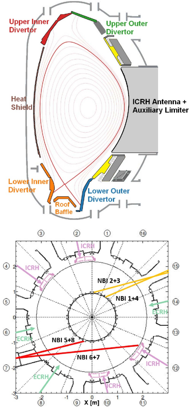
Figure 1. Top: Poloidal cross section of AUG showing all installed cooling units. The cooling units highlighted by colored areas are installed in all 16 segments. It must be mentioned that the roof baffle is aligned to the cooling unit ‘Lower Inner Divertor’. The cooling units labelled in black are installed in specific segments: the auxiliary limiters are installed in segment 6, 8, 14 and 16. The ICRH antennas are installed in segment 2, 4, 10 and 12. The tiles covering the PSL are highlighted in yellow. Bottom: Toroidal cross section of AUG indicating the position of the auxiliary heating devices NBI, electron cyclotron resonance heating (ECRH) and ICRH. The position of the ICRH antennas are added. The auxiliary limiters, installed on both side of each NBI box, are not indicated.
