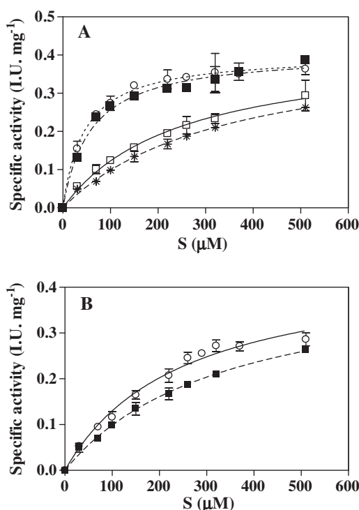
Fig. 2. Specific activity of stem bromelain towards Bz-Phe-Val-Arg-pNA substrate: (A) in Mcllvaine buffer (ethanol 12% v/v), at pH 3.2 (*), 4 (□), 5 (○) and 7 (■); (B) in two different buffer solutions at pH 3.2, containing ethanol 12% v/v: Mcllvaine (■) and tartaric buffer (○).
