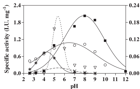
Fig. 1. Specific activity of stem bromelain in Mcllvaine buffer (25 °C) vs pH towards five model substrates. On left Y axis: (○) Bz-Phe-Val-Arg-pNA, (*) Suc-Phe-Leu-Phe-pNA, (■) Z-Arg-Arg-pNA; on right Y axis: (×) (H-Cys-pNA) 2 , (▽) Suc-Ala-Pro-Leu-Phe-pNA.
