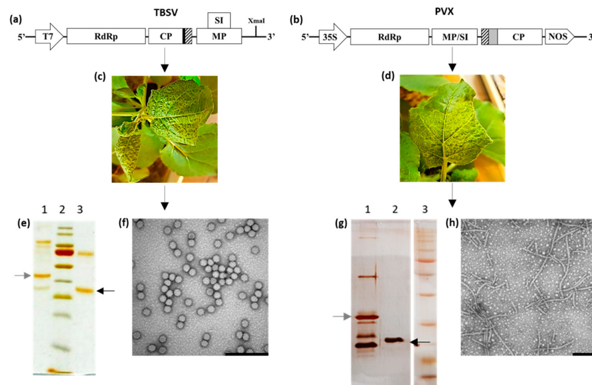
Figure 1. Production of TBSV-E-coil, TBSV-wt, and E-coil-PVX, PVX-wt NPs in plants. (a,b) Schematic diagram of genetic constructs: T7, T7 promoter; RdRp, RNA-dependent RNA polymerase; CP, coat protein; MP, movement protein; SI, silencing inhibitor; black box, linker; striped box, E-coil sequence; grey box, 2A peptide; 35S, 35S CaMV promoter; NOS, terminator sequence from A. tumefaciens nopaline synthase gene; (c,d) symptoms on systemically infected N. benthamiana leaves; (e) silver-stained SDS-PAGE of purified TBSV NPs: 1, 1 µg of E-coil-TBSV; 2, PageRuler Prestained Protein Ladder; 3, 1 µg of TBSV-wt. Black and grey arrows indicate TBSV-wt (41 kDa) and TBSV-E-coil (45 kDa) CPs, respectively; (g) silver-stained SDS-PAGE of purified PVX NPs: 1. 1 µg of E-coil-PVX; 2. 1 µg of PVX-wt; 3. Broad Range Prestained Protein Marker. Black and grey arrows indicate PVX-wt (25 kDa) and E-coil-PVX CPs (30 kDa), respectively. (f,h) Transmission Electron Microscopy images of TBSV-E-coil and E-coil-PVX purified NPs, respectively. Bars represent 200 nm.
