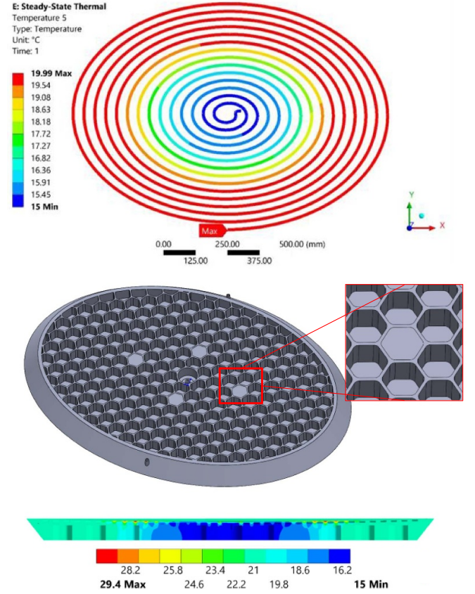
Figure 8. Focusing mirror modeling: Top: shape of the spiral channel and water temperature evaluation in steady-state. Middle: honeycomb structure on the back side. Bottom: section with temperature map calculations (units in ^{\circ}\text{C} ).
