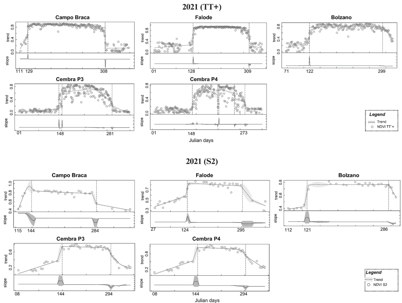
Fig. 5. 2021 phenology changepoint and trend detection resulting from the BEAST model with TT+ and S2 NDVI data in input, with associated trend line (green line) and uncertainty (grey areas). (For interpretation of the references to colour in this figure legend, the reader is referred to the web version of this article.)
