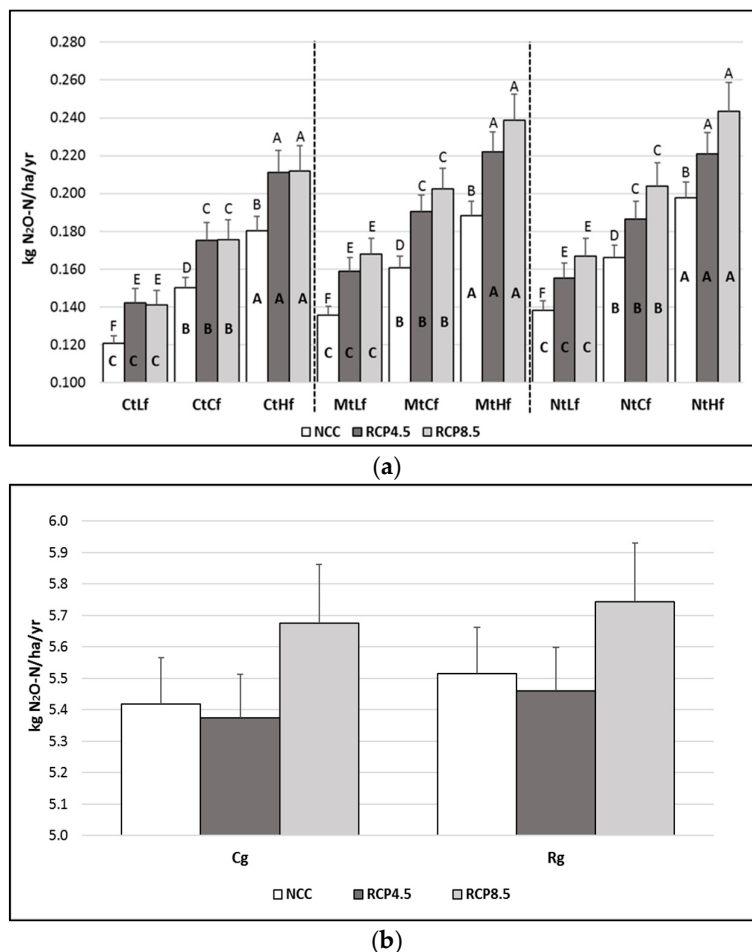
Figure 2. Denitrification–decomposition (DNDC)-modeled mean annual soil direct N 2 O fluxes ( \pm se ) from 2019 to 2089, as a result of different (a) farm management policies under diverse climate scenarios and different (b) grazing systems under diverse climate scenarios. Cf = current fertilization
