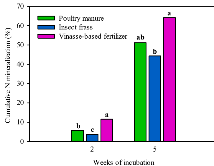
Figure 1. Mean cumulative N mineralization by fertilizer type at 2 and 5 weeks of aerobic incubation of soil: fertilizer blends. Mean square error at 2 wk = 0.53; Mean square error at 5 wk = 145.85; Coefficient of variation at 2 wk = 46.8%; Coefficient of variation at 5 wk = 26.9%; Tukey's least significant difference (5%) at 2 wk = 0.92; Tukey's least significant difference (5%) at 5 wk = 15.22. Different letters within each week of incubation indicate significant differences according to Tukey's range test (5%).
