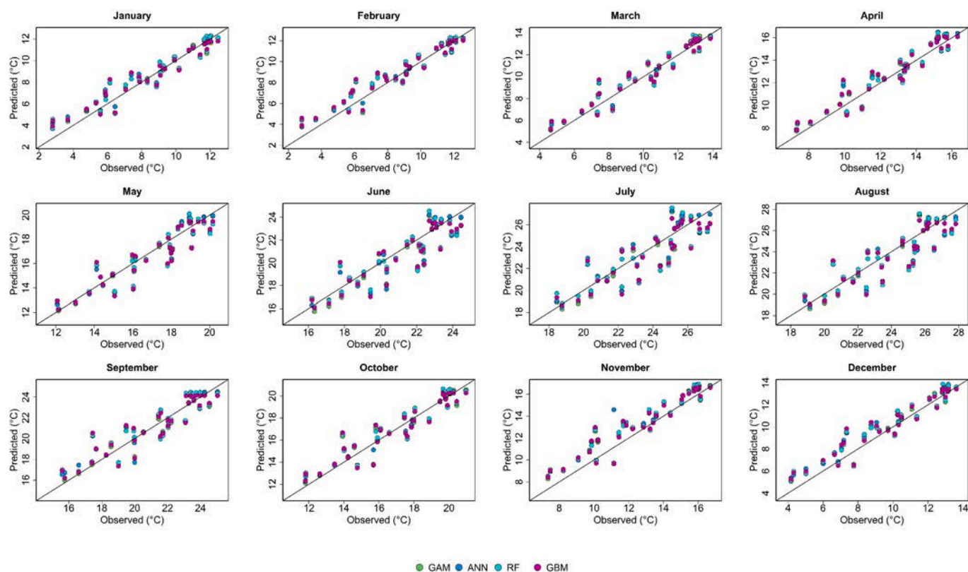
Fig. A.5. Observed monthly climates at the weather stations' locations and those predicted when downscaling WorldClim.
