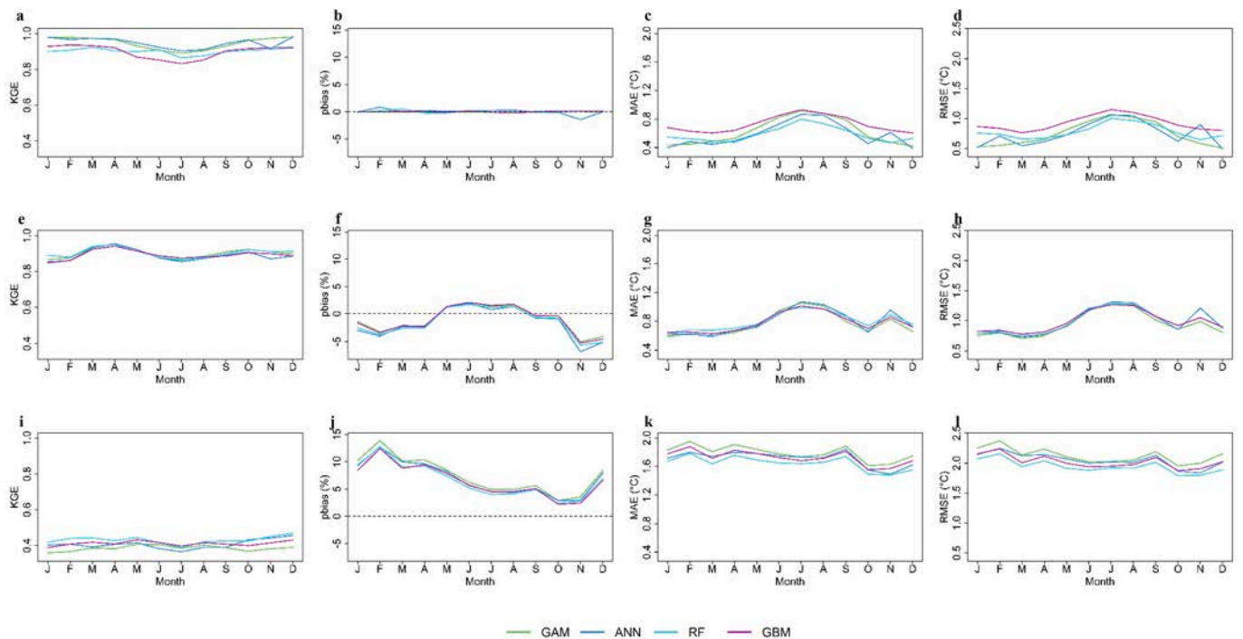
Fig. A.10. Seasonal patterns in KGE scores (first column), pbias (second column), MAE (third column), and RMSE (fourth column) that we obtained in the cross-validations when employing each algorithm to interpolate weather station data (top row) and downscale WorldClim (middle row) and CHELSA (bottom row). Model performance improves as KGE values approach 1; KGE values between 0 and 0.5 indicate poor model performance. Low pbias values reflect accurate model prediction; the optimal pbias value is 0. Model performance increases as MAE and RMSE values decrease.
