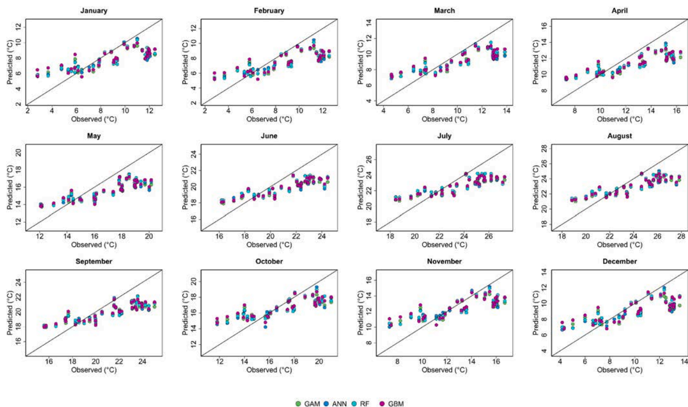
Fig. A.6. Observed monthly climates at the weather stations' locations and those predicted when downscaling CHELSA.
