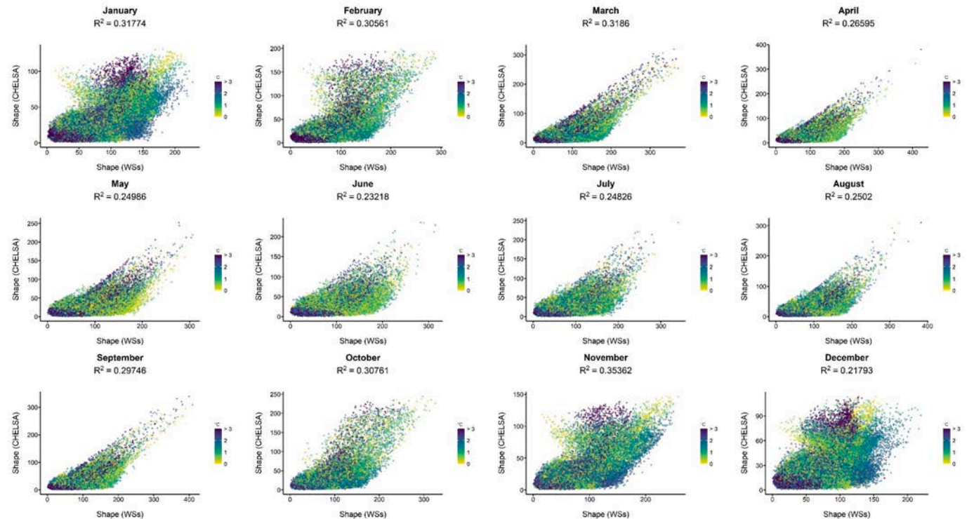
Fig. A.8. Coherence of monthly climate estimates when interpolating weather station (WS) data and downscaling CHELSA, with respect to the degree of environmental extrapolation. We quantified environmental extrapolation by calculating the Shape metric at 100,000 random points; higher Shape values indicate higher extrapolation degrees. Color gradients indicate the absolute differences between predictions under WSs interpolation and CHELSA downscaling at those 100,000 points; lighter colors indicate stronger coherence of monthly climate estimates. We capped temperature absolute differences at 3 °C for graphical purposes. R^2 values measure the degree of association between the Shape values of WSs and CHELSA.
