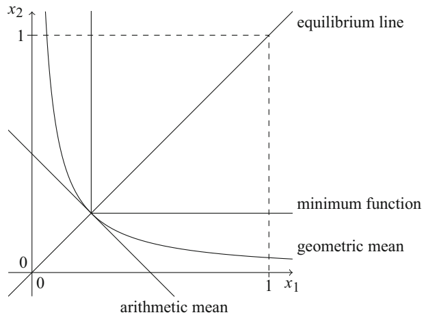
Fig. 1 Level sets of value .25 for the minimum function, the geometric mean and the arithmetic mean (for n = 2 )
