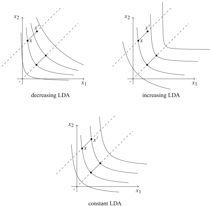
Fig. 2 Comparison of different level sets according to the LDA for typical aggregation functions
