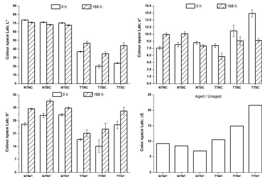
Figure 3. Chromatic coordinates L^* , a^* and b^* values, along with the standard deviation bars, and calculations of \Delta E^* for the different samples and modalities of coating application, both before and after ageing in Solar Box chamber. Untreated and uncoated wood (NTNC); untreated wood coated via brushing (NTBC); untreated wood coated via spraying (NTSC); thermally treated and uncoated wood (TTNC); thermally treated wood coated via brushing (TTBC); thermally treated wood coated via spraying (TTSC).
