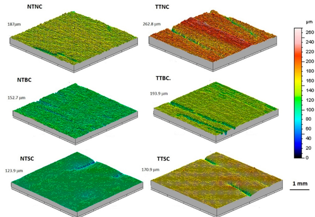
Figure 6. Roughness maps obtained for untreated (NT) and thermally treated (TT) samples uncoated (NC) and coated with the polyurethane product via brushing (BC) and spraying (SC).
