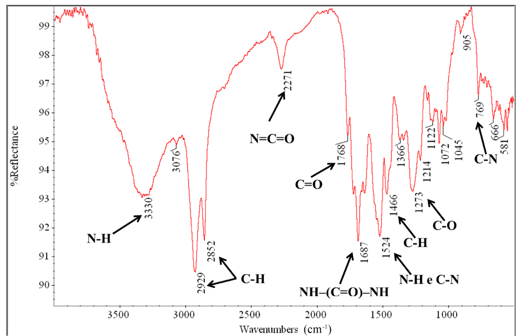
Figure 2. FTIR spectrum in the diffuse reflectance modality of the polyurethane product.
