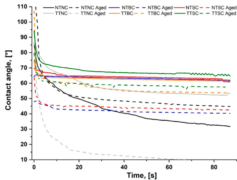
Figure 4. Contact angle trends for all samples: untreated wood that is uncoated (NTNC) and either unaged or aged; untreated wood that is coated via brushing (NTBC) and either unaged or aged; untreated wood that is coated via spraying (NTSC) and either unaged or aged; thermally treated wood that is uncoated (TTNC) and either unaged or aged; thermally treated wood that is coated via brushing (TTBC) and either unaged or aged; thermally treated wood that is coated via spraying (TTSC).
