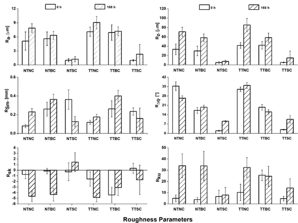
Figure 5. Roughness parameters obtained for measurements taken perpendicular to wood grain: untreated wood that was uncoated (NTNC) and either unaged or aged; untreated wood that was coated via brushing (NTBC) and either unaged or aged; untreated wood that was spray coated (NTSC) and either unaged or aged; thermally treated wood that was uncoated (TTNC) and either unaged or aged; thermally treated wood that was coated via brushing (TTBC) and either unaged or aged; and thermally treated wood spray coated (TTSC).
