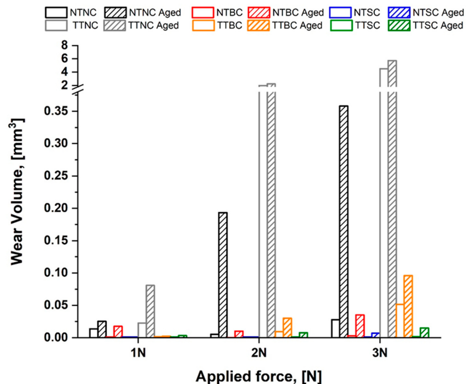
Figure 8. Wear volume average values for untreated (NT) and thermally treated (TT) samples, which were uncoated (NC) and coated with the polyurethane product via either brushing (BC) or spraying (SC), before and after 168 h of artificial ageing in Solar Box.
