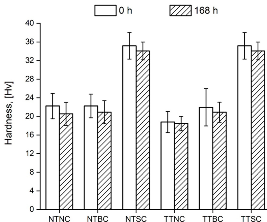
Figure 7. Micro-hardness average values for untreated (NT) and thermally treated (TT) samples, which were uncoated (NC) and coated with the polyurethane product via either brushing (BC) or spraying (SC), before and after 168 h of artificial ageing in Solar Box.
