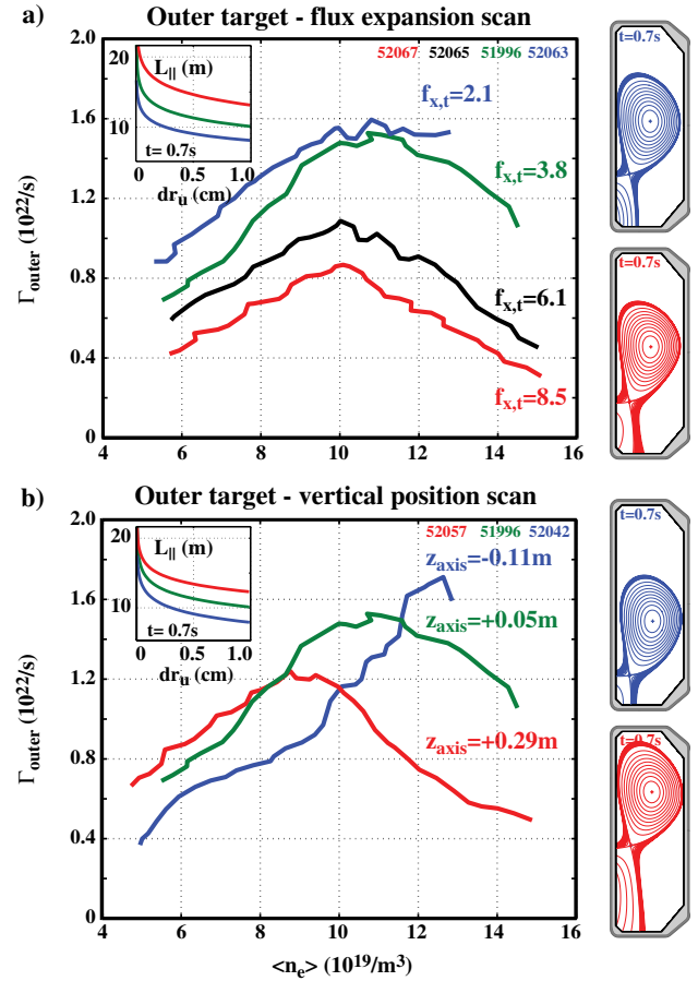
Figure 3. Density dependence of the ion current to the outer target for (a) several flux expansions ( z_{axis} \approx 0.05 m) and (b) several vertical positions ( f_{x,t} \approx 4 ). Inserts show the connection lengths.
