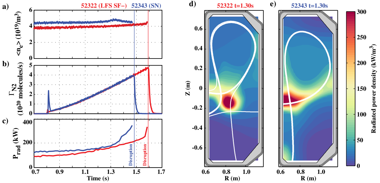
Figure 8. Evolution of (a) the average density, (b) the N 2 seeding rate and (c) the total radiated power in N 2 seeding experiments in the SF- (red) and SN (blue) configurations and comparison of the radiated power density in (d) the SF- and (e) the SN configurations for the same seeding rate ( \Gamma_{N2} = 2.8 \times 10^{20} molecules s -1 ).
