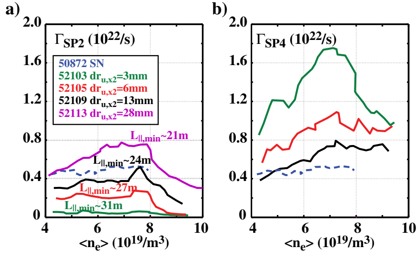
Figure 7. Density dependence of the ion currents to (a) SP2 and (b) SP4 in LFS SF – configurations with various separations of the x -points.
