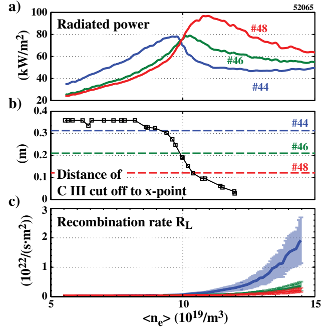
Figure 2. Density dependence of (a) radiation emission along the chords shown in figure 1(a) and (b) the poloidal distance of the C III cut-off from the x-point and (c) the line integrated recombination rate R_L along chords similar to the bolometer chords estimated from DSS measurements of the Balmer spectrum.
