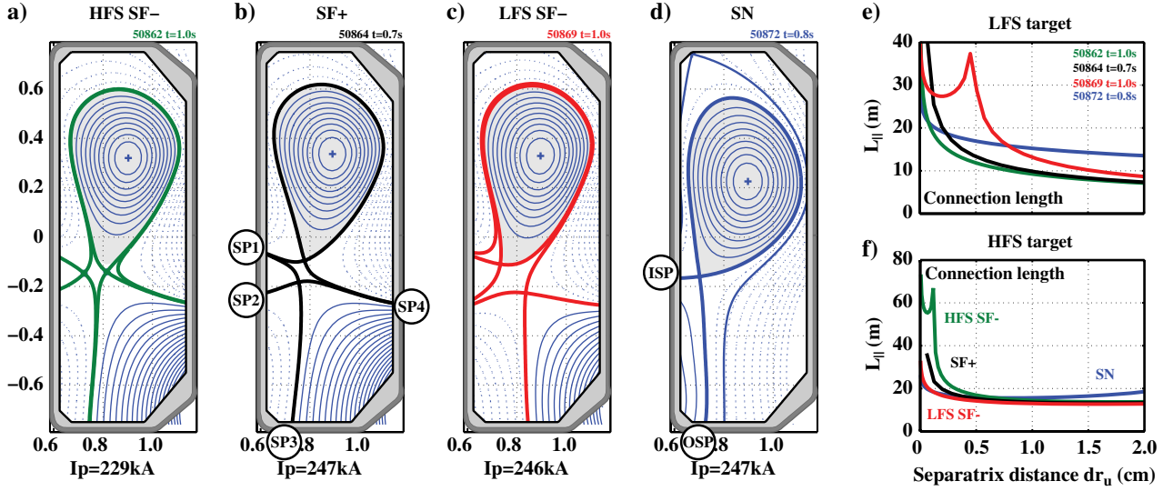
Figure 6. Realised SF configurations (a)–(c) and SN reference (d) together with the connection length from the outboard mid-plane downwards (e) and upwards (f) to the targets. Labels in (b) and (d) indicate the customary notation of strike points.
