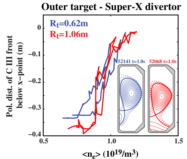
Figure 5. Movement of the C III cut-off front in density ramps ( B_T = 1.42 T, I_p = 340 kA) with different outer target radii [6]. Reproduced from [6]. © 2017 Ecole Polytechnique Federale de Lausanne. CC BY 3.0.
