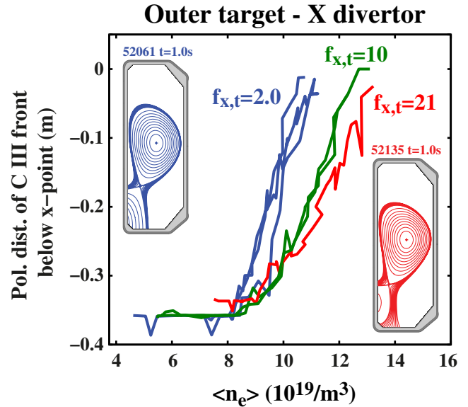
Figure 4. Movement of the C III cut-off front in density ramps ( B_T = 1.42 T, I_p = 340 kA) with different flux flaring at the outer target [6]. Reproduced from [6]. © 2017 Ecole Polytechnique Federale de Lausanne. CC BY 3.0.
