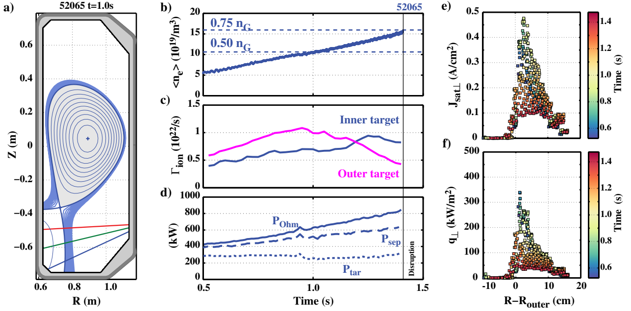
Figure 1. (a) Standard TCV divertor configuration ( B_T = 1.42 T, I_p = 340 kA, q_{95} = 2.5 ) and evolution of (b) the line averaged density \langle n_e \rangle , (c) total ion fluxes \Gamma_{ion} to the inner and outer targets and (d) Ohmic heating power P_{Ohm} , power crossing the separatrix P_{sep} \approx P_{Ohm} - P_{rad,core} and power at the wall P_{tar} \approx P_{Ohm} - P_{rad} in an Ohmically heated density ramp experiment. Also shown are the (e) ion current j_{sat,\perp} and (f) heat flux profiles q_{\perp} measured with Langmuir probes at the outer target.
