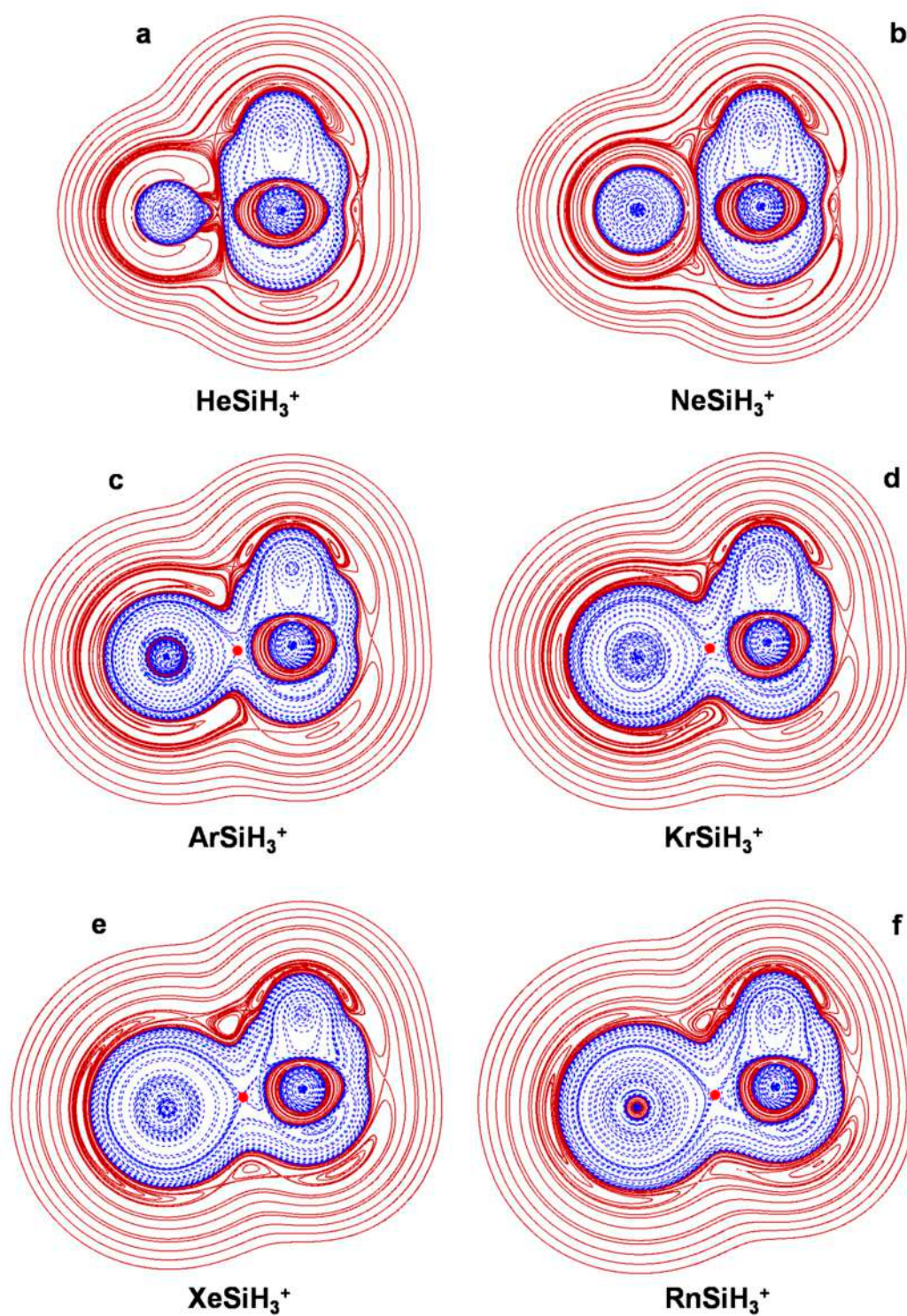
Figure 2. 2D plots of H(r) in the symmetry plane of (a) \text{HeSiH}_3^+ ; (b) \text{NeSiH}_3^+ ; (c) \text{ArSiH}_3^+ ; (d) \text{KrSiH}_3^+ ; (e) \text{XeSiH}_3^+ ; (f) \text{RnSiH}_3^+ (solid/brown and dashed/blue lines correspond, respectively, to positive and negative values). The red dots represent the HCPs.
