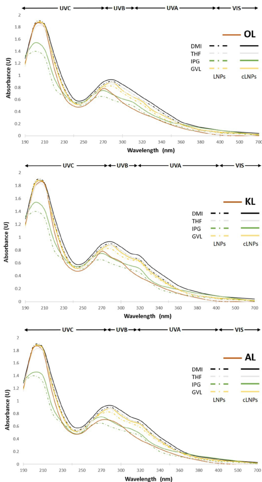
Figure 3. UV absorbance capacity of LNP and cLNP. The analysis was performed with the appropriate sample (0.05 mg/mL) in the range from 190 to 700 nm at 25 °C under gentle stirring. Native amorphous lignin was used as a reference. Both UV-B and UV-A ranges are reported.
