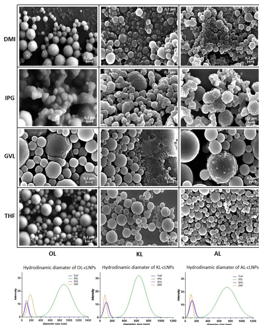
Figure 1. SEM images (upper panel) and DLS diagrams (lower panel) of KL-cLNPs, OL-cLNPs, and AL-cLNPs. The SEM image shows that the grid allows the connection of different types of lignin with different types of primary solvents used in the nanoprecipitation process.
