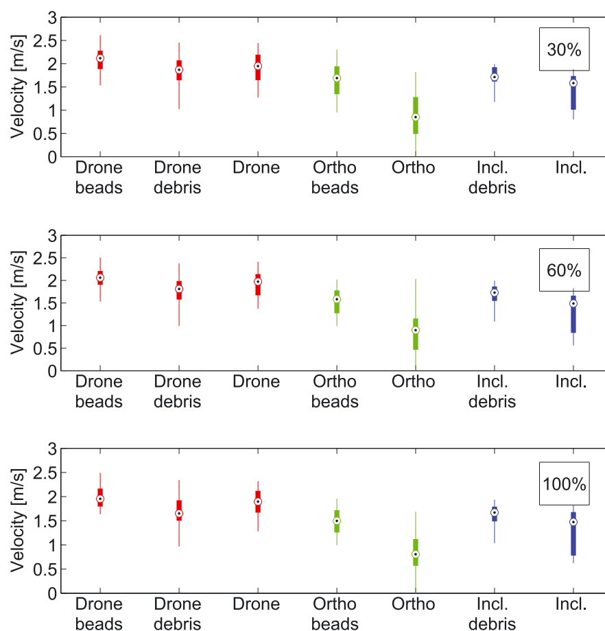
Figure 7. Artificial channel: velocity range values for cross sections in the shared subarea for each experimental condition. Markers indicate medians computed over the experimental replicates. The edges of the box indicate the 25th and 75th percentiles, and the whiskers extend to extreme data points that are not outliers. For each replicate, velocity range values are computed considering 30 % (top graph), 60 % (central graph), and 100 % (bottom graph) of the image sequences
