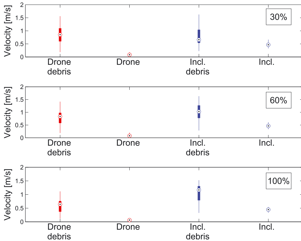
Figure 12. Diverging segment: velocity range values for cross sections in the shared subarea for each experimental condition. Markers indicate medians computed over the experimental replicates. The edges of the box indicate the 25th and 75th percentiles, and the whiskers extend to extreme data points that are not outliers. For each replicate, velocity range values are computed considering 30 % (top graph), 60 % (central graph), and 100 % (bottom graph) of the image sequences
