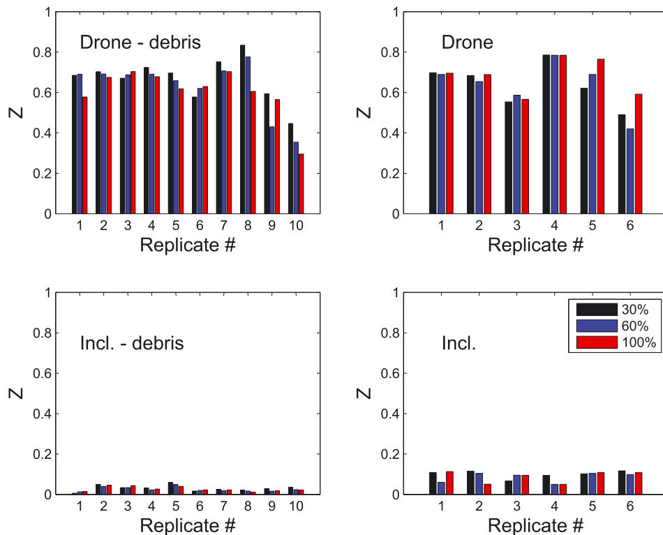
Figure 9. Diverging segment: Z values for each experimental condition. In the top row, drone data (drone) are reported in case of debris and without tracers. In the bottom row, data are showed for the fixed-inclined configuration (incl.) in case of debris and without tracers. For each replicate, Z values are computed considering 30 % (black bars), 60 % (blue bars), and 100 % (red bars) of the image sequences
