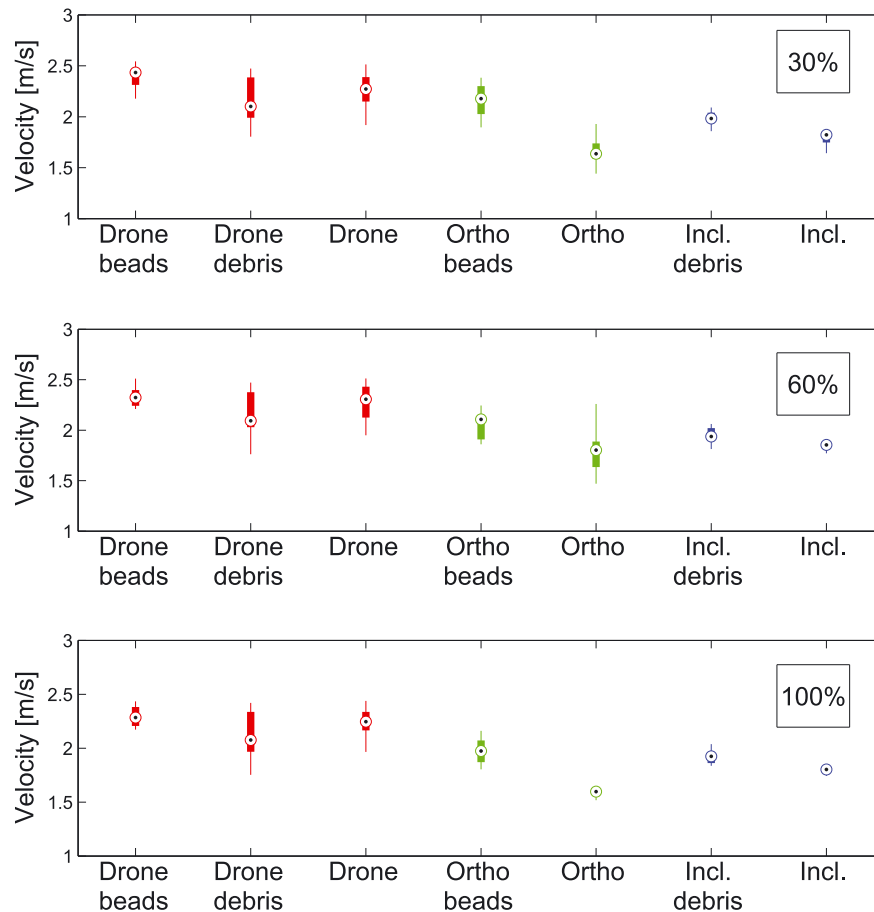
Figure 6. Artificial channel: maximum velocity values in the shared subarea for each experimental condition. Markers indicate medians computed over the experimental replicates. The edges of the box indicate the 25th and 75th percentiles, and the whiskers extend to extreme data points that are not outliers. For each replicate, maximum velocity values are computed considering 30 % (top graph), 60 % (central graph), and 100 % (bottom graph) of the image sequences
