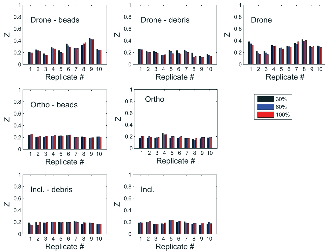
Figure 3. Artificial channel: Z values for each experimental condition. In the top row, drone data (drone) are reported in case of beads, debris, and without tracers. In the central row, data are illustrated for the fixed-ortho configuration (ortho) in case of beads and without tracers. In the bottom row, data are reported for the fixed-inclined configuration (incl.) in case of debris and without tracers. For each replicate, Z values are computed considering 30 % (black bars), 60 % (blue bars), and 100 % (red bars) of the image sequences
