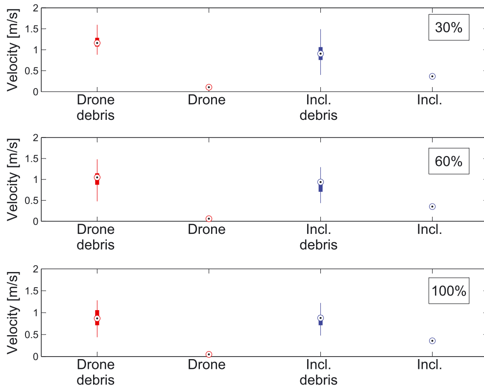
Figure 11. Diverging segment: maximum velocity values in the shared subarea for each experimental condition. Markers indicate medians computed over the experimental replicates. The edges of the box indicate the 25th and 75th percentiles, and the whiskers extend to extreme data points that are not outliers. For each replicate, maximum velocity values are computed considering 30 % (top graph), 60 % (central graph), and 100 % (bottom graph) of the image sequences
