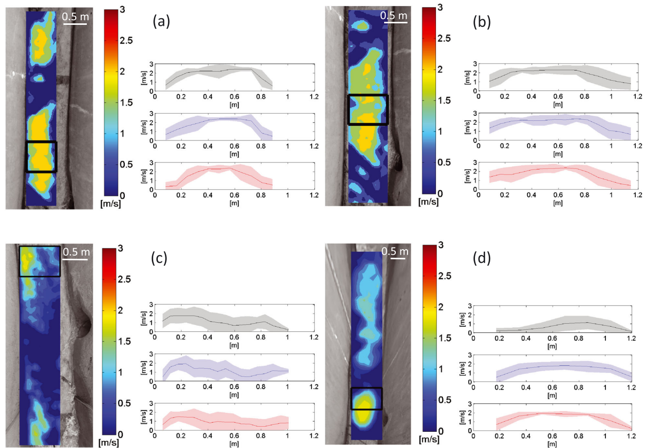
Figure 2. Representative surface flow observations for experiments conducted in the artificial channel. (a) Time-averaged surface flow velocity map and cross-sectional profiles generated from drone data and in case of artificial beads as tracers. (b) Time-averaged surface flow velocity map and cross-sectional profiles generated from drone data and in case of natural debris as tracer. (c) Time-averaged surface flow velocity map and cross-sectional profiles generated from the fixed-ortho configuration data and in case of artificial beads as tracers. (d) Time-averaged surface flow velocity map and cross-sectional profiles generated from the fixed-inclined configuration data and in case of natural debris as tracer. Black boxes indicate the subarea shared by all experimental configurations
