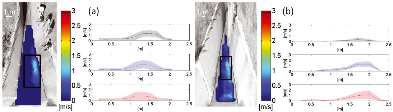
Figure 8. Representative surface flow observations for experiments conducted in the diverging segment. (a) Time-averaged surface flow velocity map and cross-sectional profiles generated from drone data in case of natural debris as tracer. (b) Time-averaged surface flow velocity map and cross-sectional profiles generated from data captured through the fixed-inclined configuration in case of natural debris as tracer
