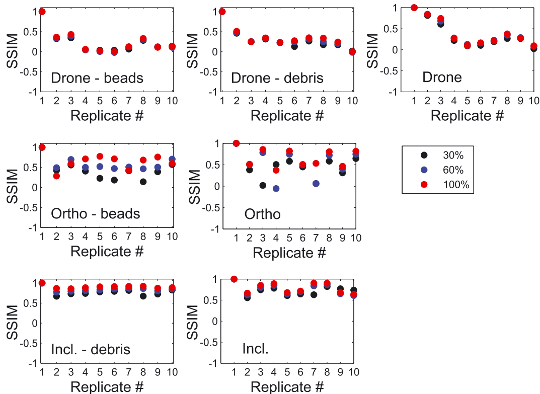
Figure 5. Artificial channel: structural similarity index (SSIM) values for each experimental condition. In the top row, SSIM values are displayed for drone data (drone) in case of beads, debris, and without tracers. In the central row, SSIM values are reported for the fixed-ortho configuration (ortho) in case of beads and without tracers. In the bottom row, SSIM values are shown for the fixed-inclined configuration (incl.) in case of debris and without tracers. For each replicate, SSIM values are computed considering 30 % (black markers), 60 % (blue markers), and 100 % (red markers) of the image sequences
