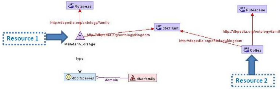
Fig. 4. D_1 : an RDF dataset about Mandarin Orange and Coffea. The graph matches the left-hand data pattern given in Experiment 2 in Section 2.1, by binding x to Resource 1
