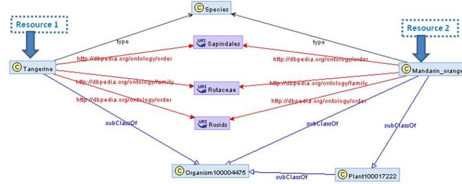
Fig. 2. D_1 : an RDF dataset about Mandarin Orange and Tangerine. The graph matches the left-hand data pattern given in Experiment 1 in Section 2.1, by binding x to Resource 2
