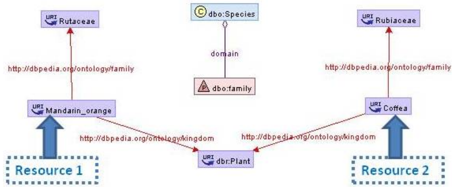
Fig. 5. D_2 : a dataset logically equivalent to the one in Figure 4. The graph matches the right-hand data pattern given in Experiment 2 in Section 2.1, by binding x to Resource 1
