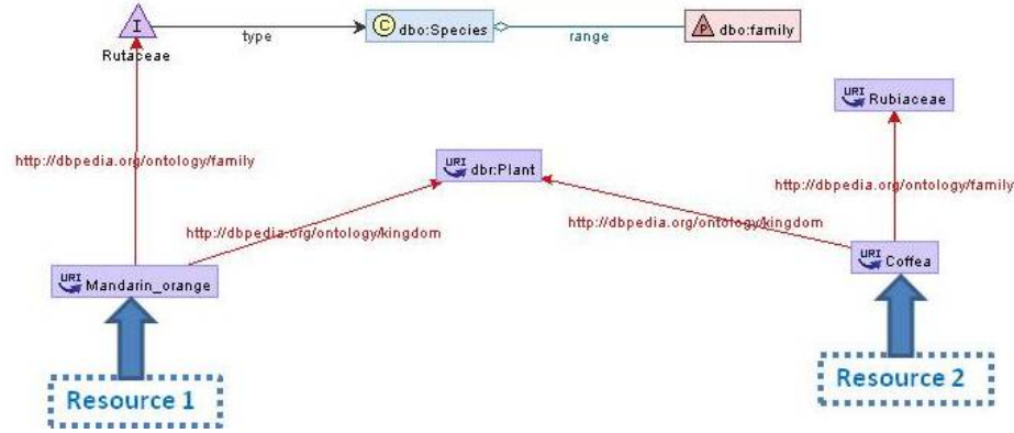
Fig. 6. D_1 : an RDF dataset about Mandarin Orange and Coffea. The graph matches the left-hand data pattern given in Experiment 3 in Section 2.1, by binding x to Resource 1
