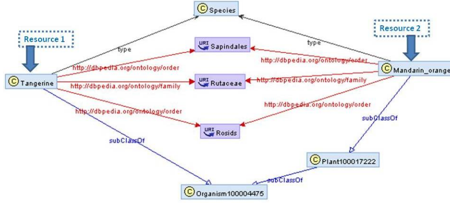
Fig. 3. D_2 : a dataset logically equivalent to the one in Figure 2. The graph matches the right-hand data pattern given in Experiment 1 in Section 2.1, by binding x to Resource 2 .
