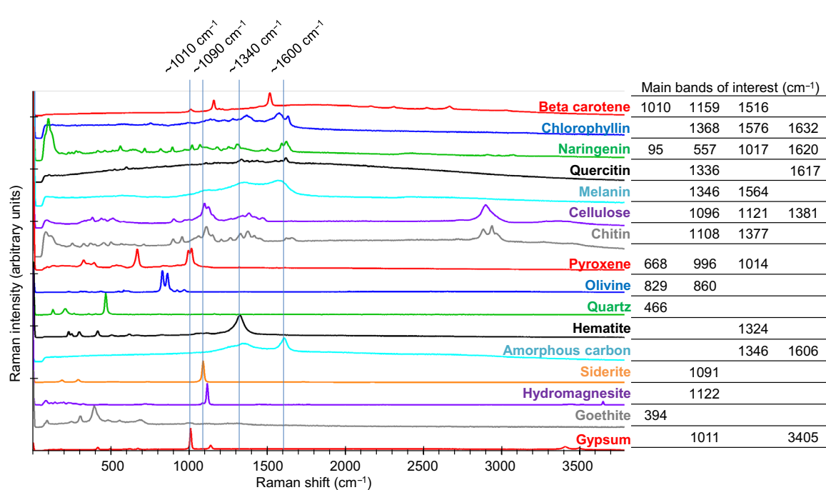
Fig. 1. Raman spectra of investigated biogenic compounds and martian regolith analogs. Stacked Raman spectra recorded at 532-nm excitation wavelength with overlapping regions, indicated by blue lines, and main bands of interest (details in fig. S1).
