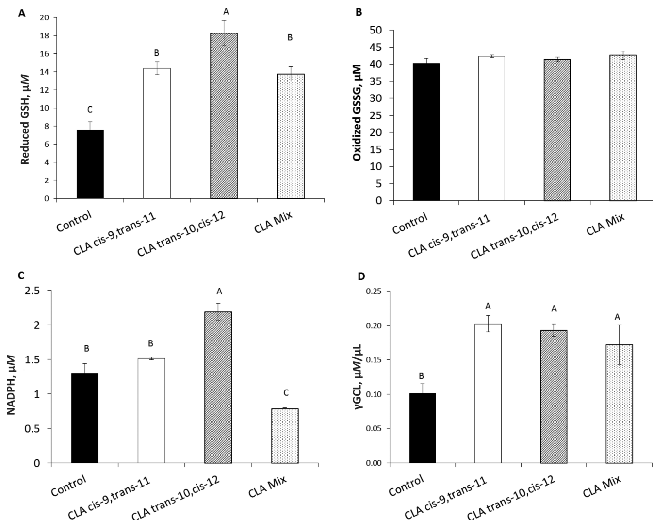
Figure 1. Intracellular concentrations of reduced (GSH; A) and oxidized (GSSG; B) glutathione, NADPH (C), and \gamma -glutamate cysteine ligase ( \gamma\text{GCL} ; D) activity in BME-UV1 cells after 48 h of CLA isomer exposure. Data are reported as least squares means \pm standard error of the mean ( n = 6 ). Significant differences between the control group and treatments and among treatments are represented by different letters ( ^{A,B}P < 0.01 ). CLA mix = 50% cis -9, trans -11/50% trans -10, cis -12.
