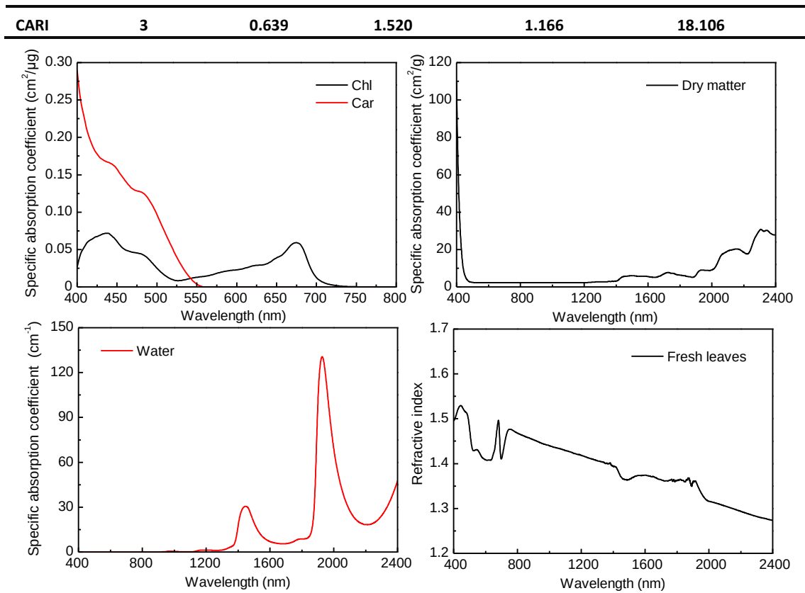
Fig. 1. Specific absorption coefficient of pigments in vivo, dry matter and water, and refractive index for PROSPECT-5.
