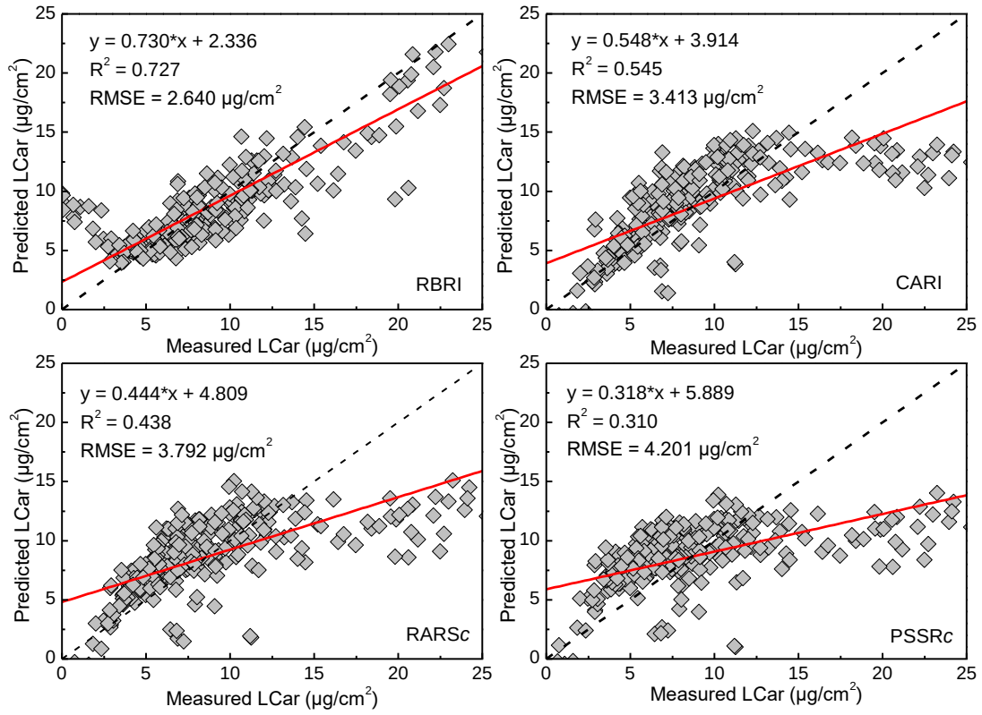
Fig. 4. Scatterplots of measured LCar versus predicted LCar for spectral indices with ANGERS dataset (n = 276). Dashed lines indicate 1:1 lines.
