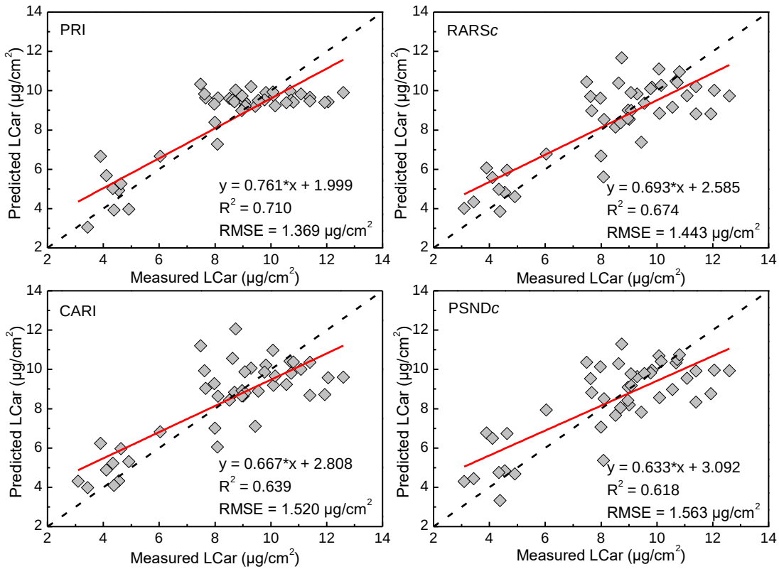
Fig. 5. Scatterplots of measured LCar versus predicted LCar for spectral indices with leaf level experimental data (n = 44). Dashed lines indicate 1:1 lines.
