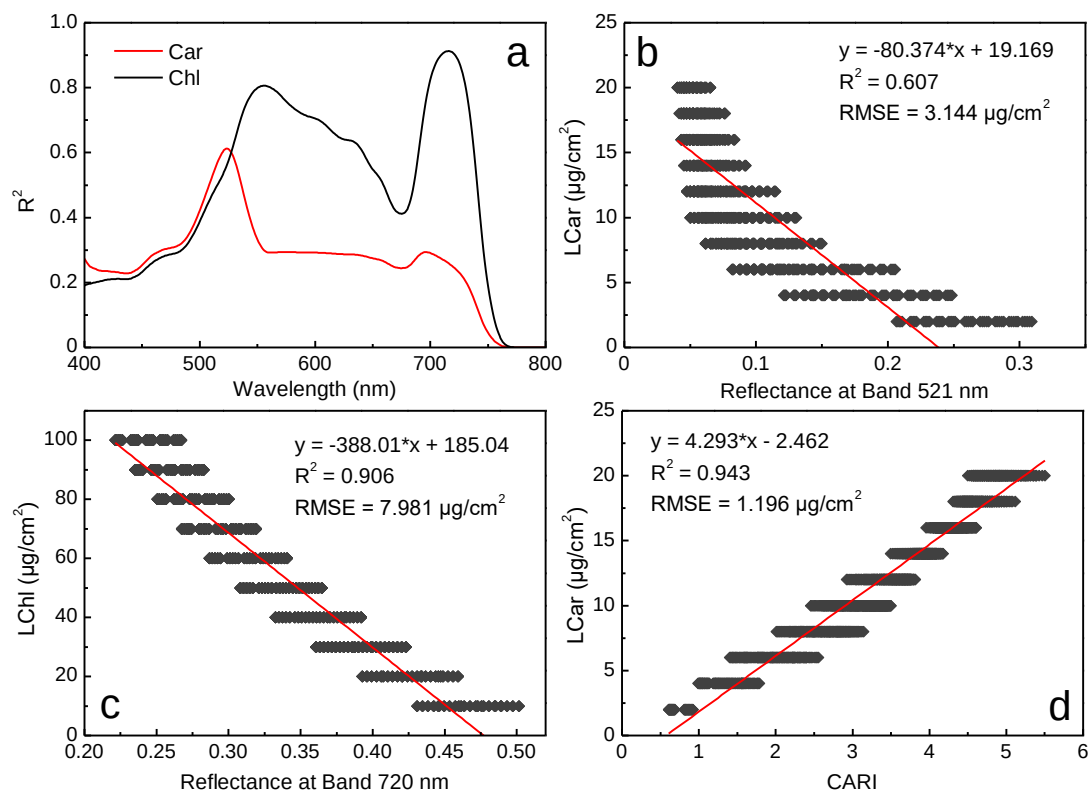
Fig. 2. (a) R^2 curves for LCar (LChl) versus leaf reflectance within the wavelength range from 400 to 800 nm. (b) Correlation between band 521 nm and LCar. (c) Correlation between band 720 nm
