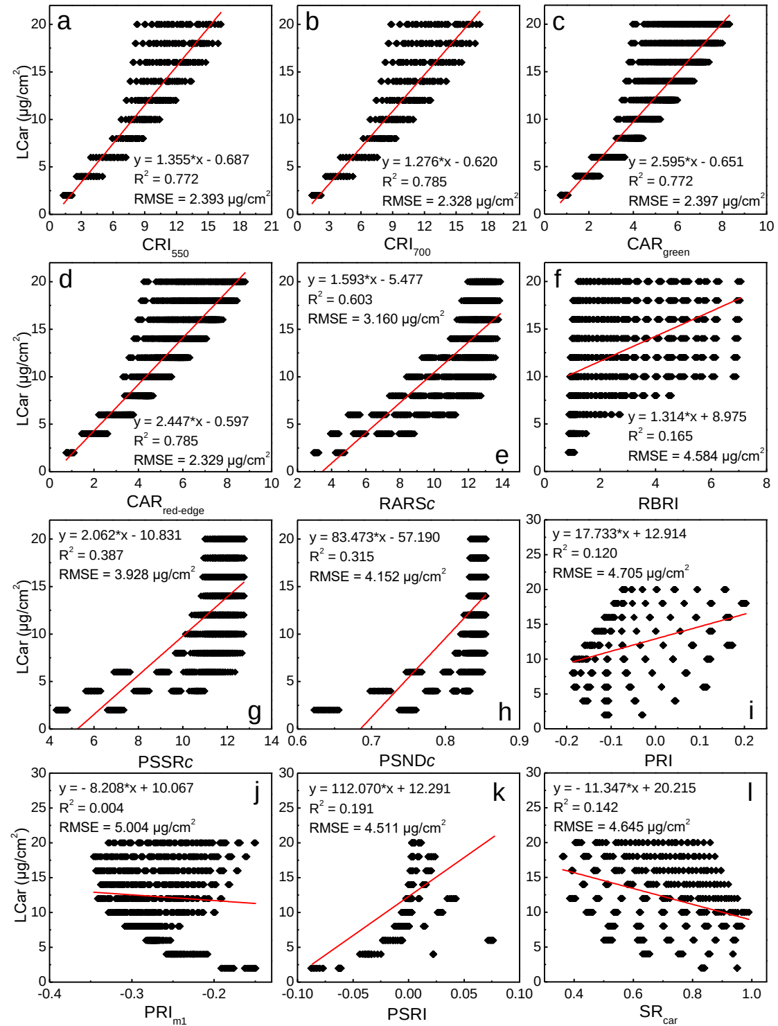
Fig. 3. Relationships between published spectral indices and leaf carotenoids content from leaf level data simulated with PROSPECT-5 (n = 1700).
