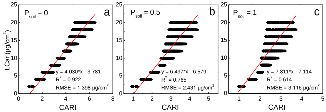
Fig. 7. Relationships between CARI and LCar using canopy reflectance simulations with LAI value fixed to 1 at different soil moisture levels. P_{\text{soil}} value set as (a) 0, (b) 0.5 and (c) 1. ALL other parameters for 4SAIL were fixed based on Table. 3 ( n = 1700 ).
