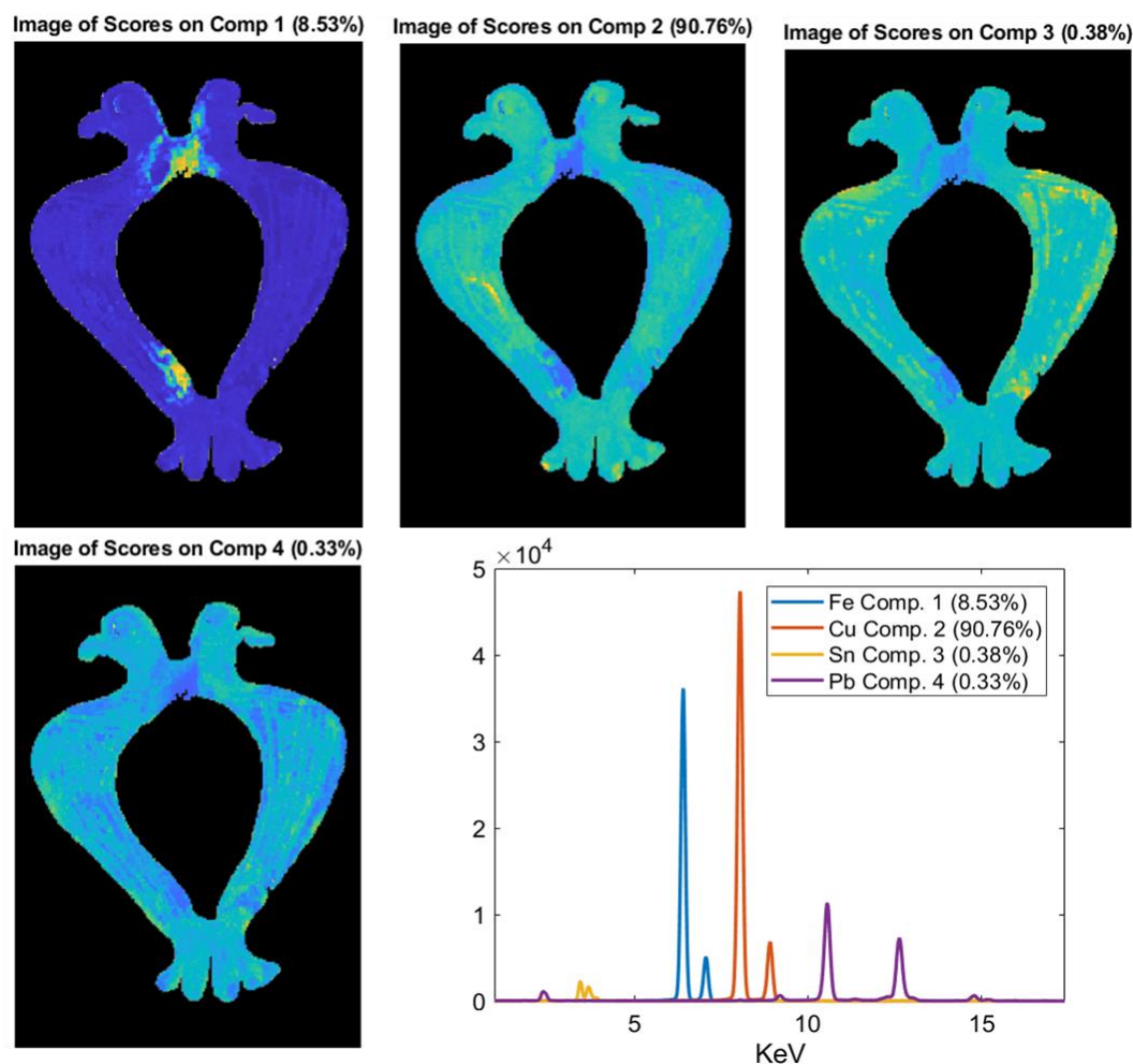
Figure 14. MCR analysis on the XRF spectra of the zoomorphic fibula 4021_12. This analysis highlights the difference in composition between the copper-based alloy (Comp. 2) and the parts rich of iron (Comp. 1).
