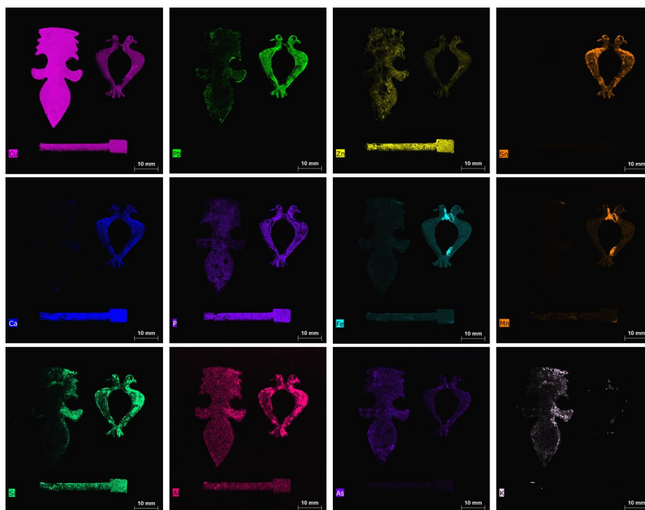
Figure 8. Elemental maps for the detected elements of applique, zoomorphic fibula, and spatula. The maps of S and Ti are not shown due to the extremely low contents of these two elements.
