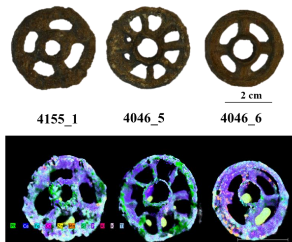
Figure 3. Photographs of the three ornamental jewellery objects and the XRF mapping of the detected elements.
