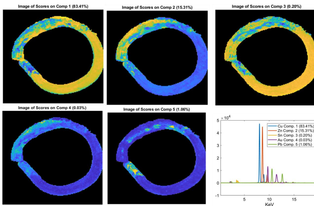
Figure 12. Multivariate curve resolution (MCR) analysis on the XRF spectra of the object 5085_6. Cu and Sn are uniformly distributed in the alloy (Comp. 1 and Comp. 3), while Zn (Comp. 2) is concentrated in a defined area. Traces of gold are confirmed (Comp. 4), and in a little area of the surface, a high concentration of Pb is obtained (Comp. 5).
