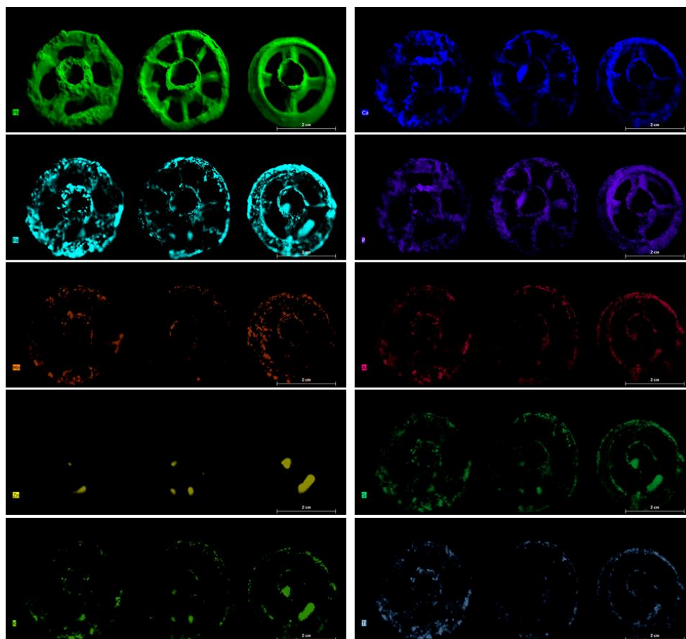
Figure 4. Elemental maps for the detected elements of the three ornamental jewellery items. The Cu map is not shown due to the extremely low content of this element.
