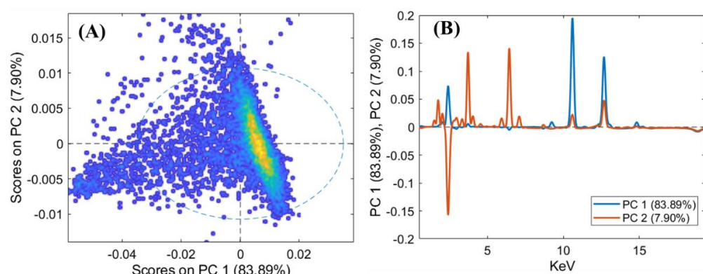
Figure 9. Principal component analysis (PCA) score plot of the XRF spectra (A) and the loadings of PC1 and PC2 (B) for the three lead wheels (i.e., ornamental jewellery, talismans, or little toys).
