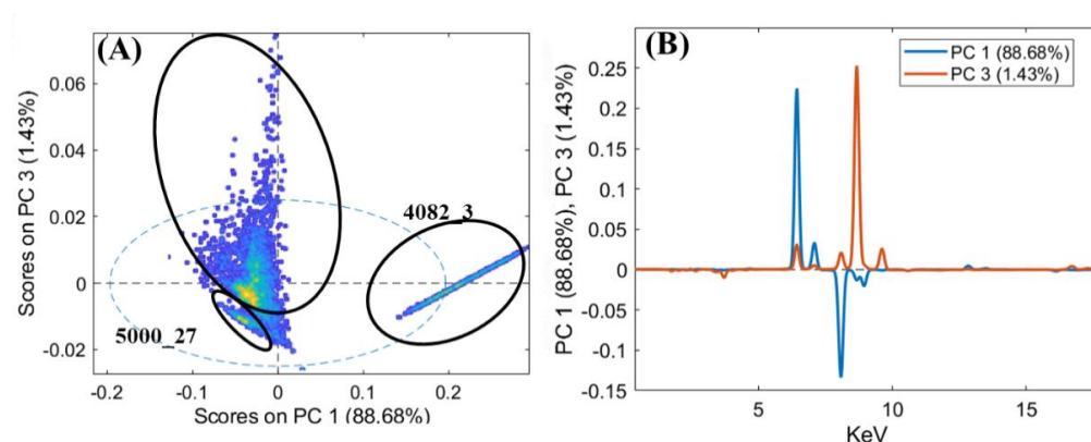
Figure 10. PCA score plot of the XRF spectra (A) and the loadings of PC1 and PC3 (B) for the fibulae (4003_7, 4025_4, 5000_27, and 5050_4), earrings (5079_5 and 5085_6), and ring (4082_3).
