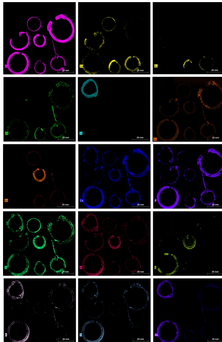
Figure 6. Elemental maps for all detected elements of fibula/ring/earring group.
