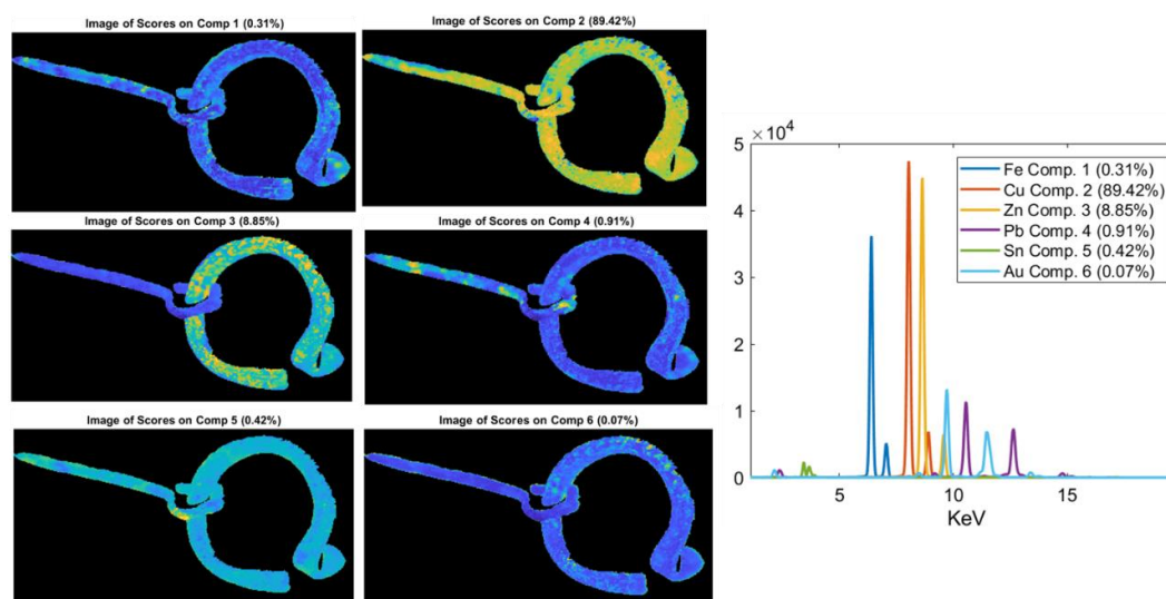
Figure 13. MCR analysis on the fibula 5123_45, the only one having the prong. Zn is uniformly distributed on the object's surface (Comp. 3), while traces of gold are confirmed (Comp. 6), and a high Pb content is visible in the prong (Comp. 4).
