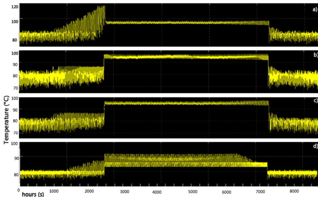
Figure 15. Results of the temperature trend of the network tank for different sizes; (a) 60 m 3 ; (b) 90 m 3 ; (c) 120 m 3 ; and (d) 150 m 3 .
