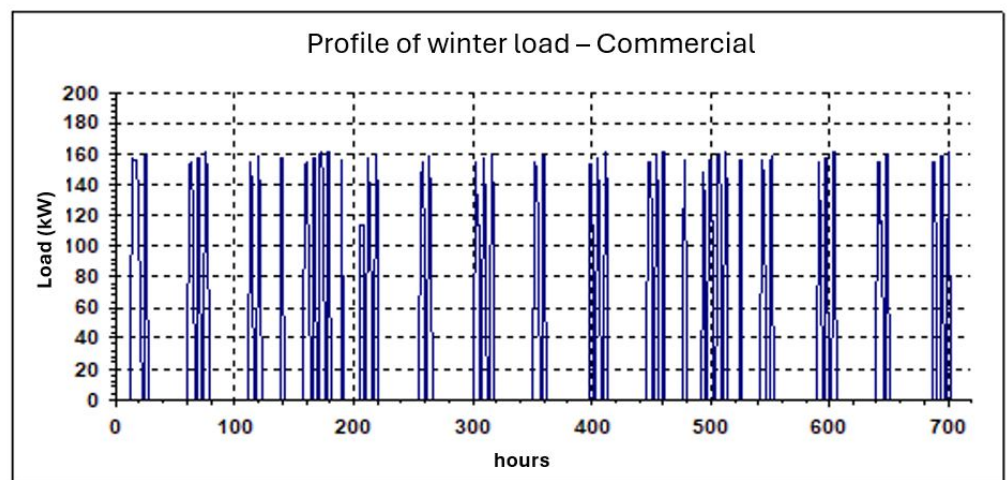
Figure 3. Example of commercial building's winter load profile.
