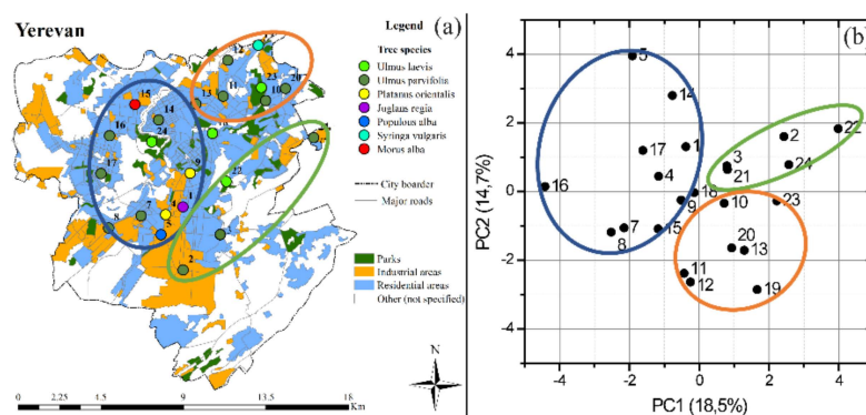
Figure 5. Yerevan territory tree leaves and soil element contents PCA results-spatial representation (a) and factor scores per case (b).
