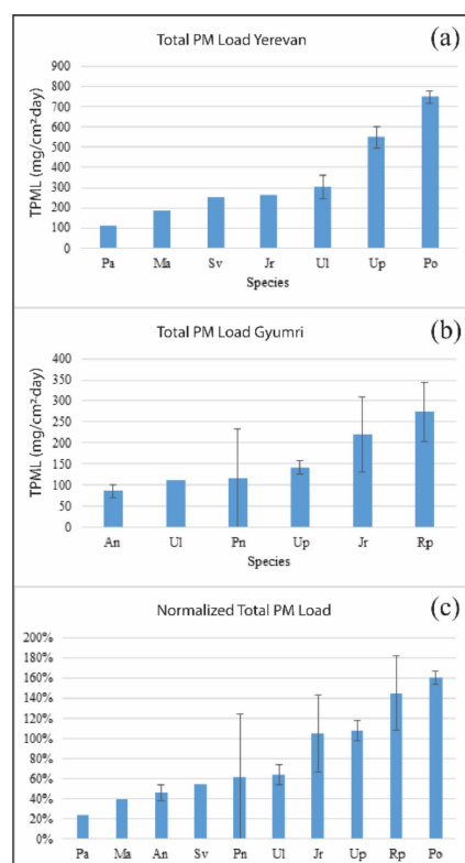
Figure 4. Average total PM load (TPML) per tree species in Yerevan (a) and Gyumri (b). The data from the two cities, properly normalized by the city average TPML, are averaged and combined in panel (c). Error bars represent standard deviations.
