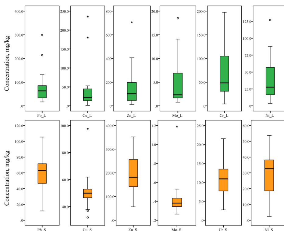
Figure 3. Box plots of studied PTE concentration in Gyumri's tree leaf-deposited PM and soil (o—outliers and *—extreme values).
