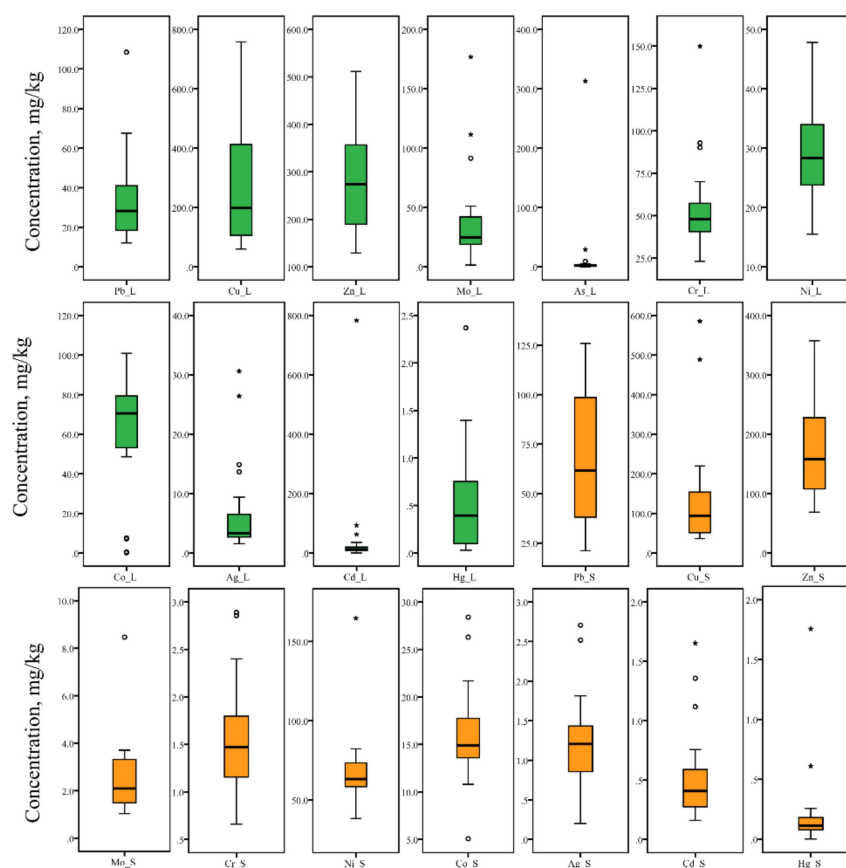
Figure 2. Box plots of studied PTE concentration in Yerevan’s tree leaf-deposited PM and soil (o—outliers and *—extreme values; for a better visualization, the extremely high content of Mo in sampling site 6 was removed).
