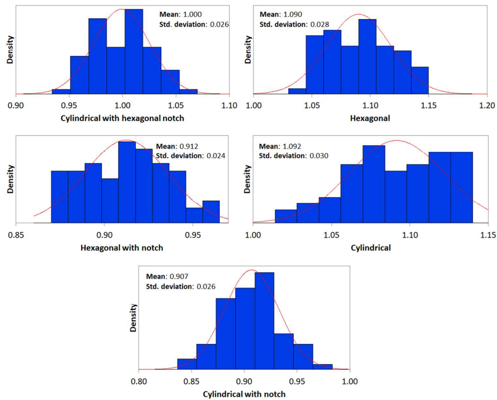
Figure 9. Distribution fitting analysis for the corrective factors
