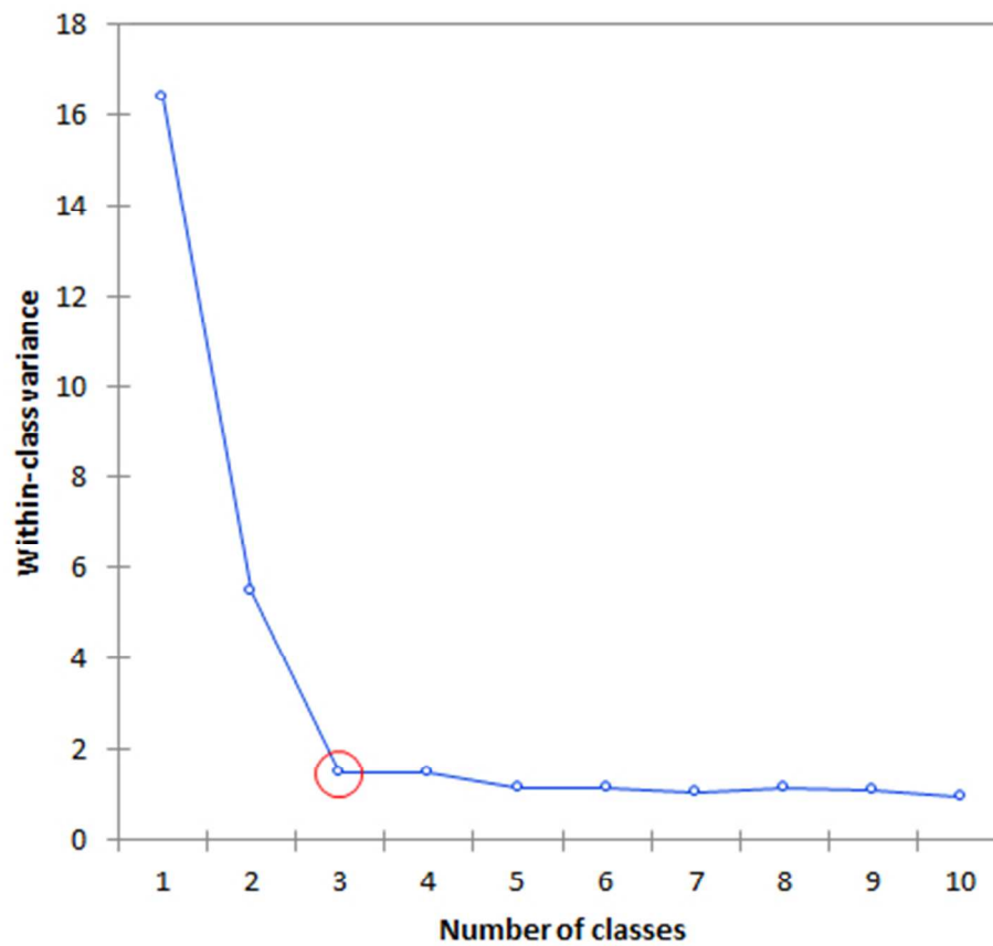
Figure 5. Within-cluster sum of square (WSS) for screw diameter clustering. The red circle indicates the optimal number of clusters (elbow method)
