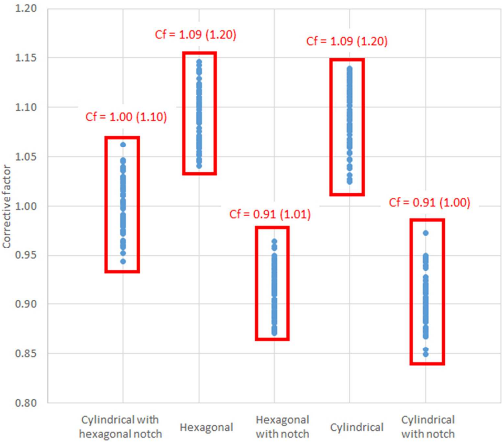
Figure 8. Corrective factors for screw head type (cluster view). Within brackets the normalized corrective factors
