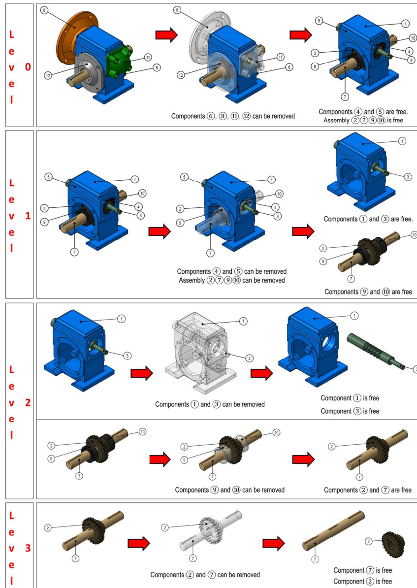
Figure 3. Disassembly levels for the gear reducer example
