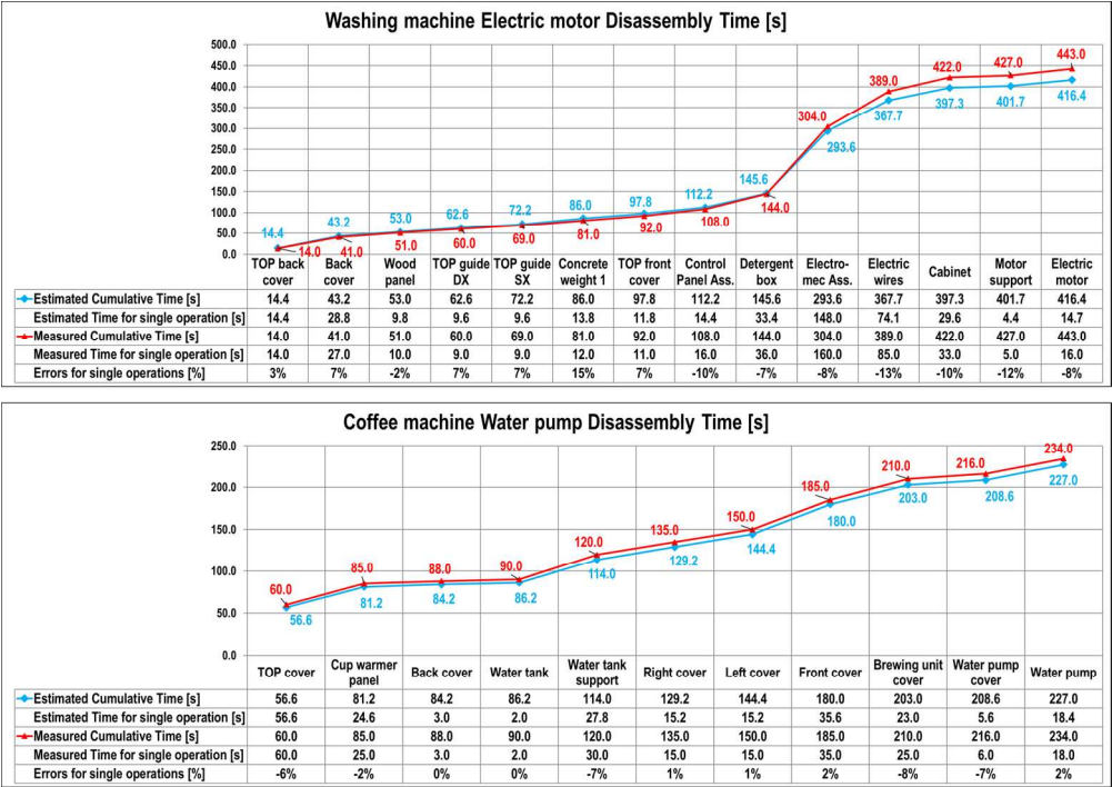
Figure 12. Cumulative disassembly time graph for the washing machine electric motor and for the coffee machine water pump
