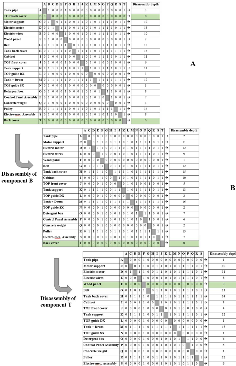
Figure 11. 'Level' matrices for the washing machine: (A) initial matrix, (B) reduced matrix after the disassembly of component B, (C) reduced matrix after the disassembly of component B and T
