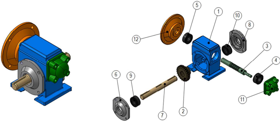
Figure 2. Exploded view of the gear reducer example
