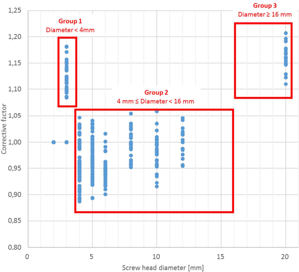
Figure 6. Screw diameter clustering (k-means algorithm) 82x78mm (300 x 300 DPI)
