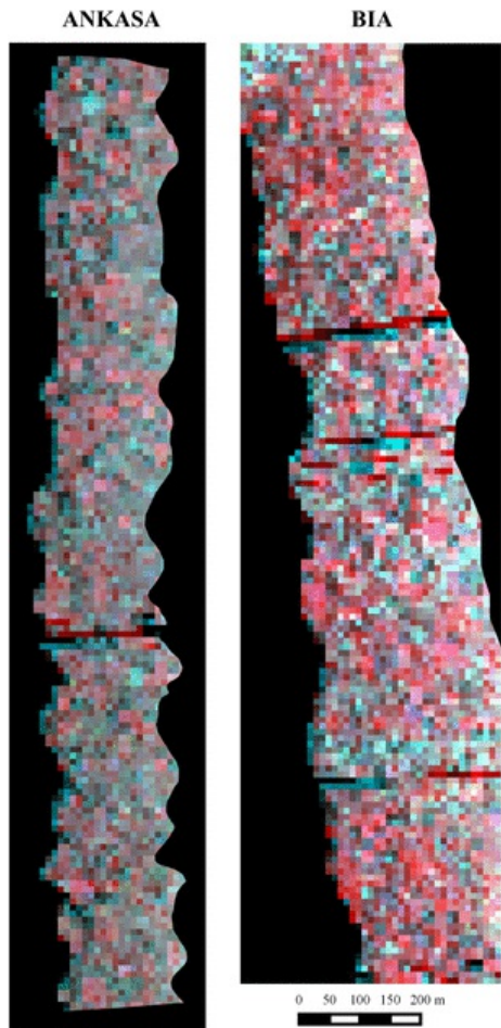
Figure 3: Simulated Sentinel-2 data derived from hyperspectral strips collected in Ankasa and Bia Conservation areas. False color composite of bands 8 (R), 3 (G), 2 (B).
