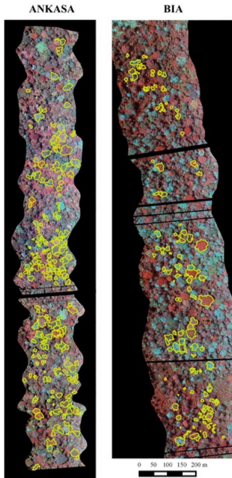
Figure 2. Hyperspectral data collected over Ankasa and Bia Conservation Areas in a false color composite of 829 nm (R), 604 (G), and 465 (B) bands. The yellow polygons represent the delineated crown species.
