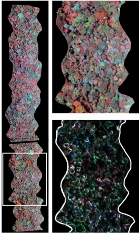
Figure 4-Fig. 4 Ankasa hyperspectral data. On the left hand the hyperspectral strip over Ankasa Conservation Area: false color composite of 829-nm (R), 604 (G), and 465 (B) bands. On the upper right hand a zoom of the left image for the white-delineated region; on the lower right hand the same regions is shown using a false color composite of variance textures from bands 1 (R), 5 (G), and 6 (B) which highlight crowns edges.
