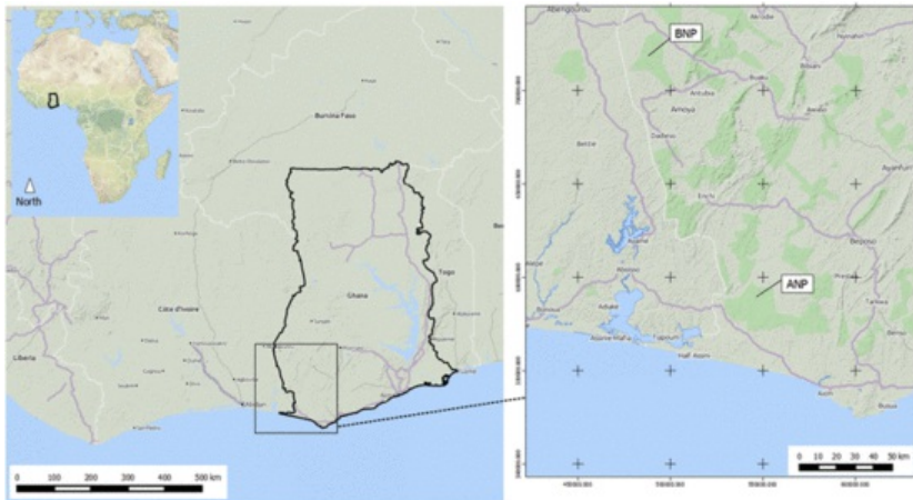
Figure 1. Fig. 1 Location of Ankasa (ANP) and Bia (BNP) Conservation Areas.
